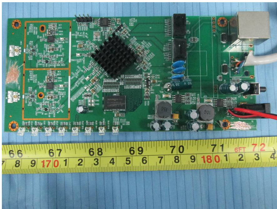
EUT –Main Board 1 Top View (Model: LKV388A)
