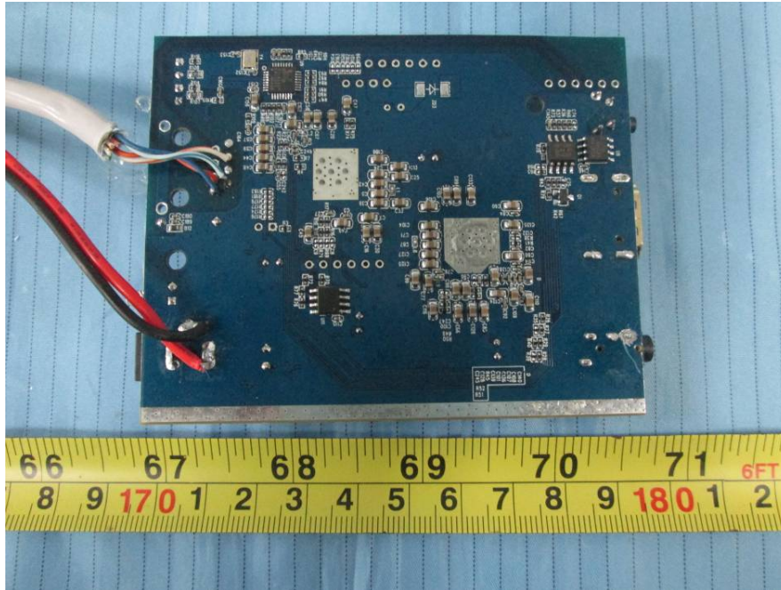
EUT –Main Board 2 Bottom View (Model: LKV388A)
