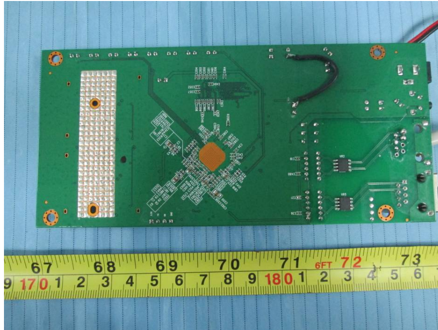
EUT –Main Board 1 Bottom View (Model: LKV388A)
