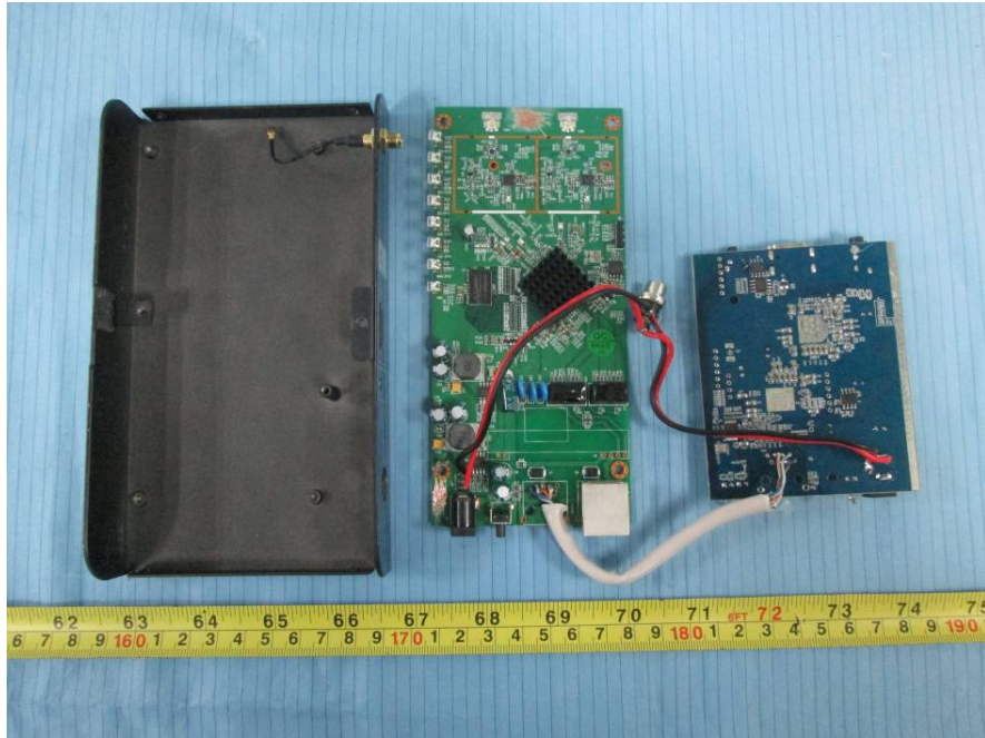
EUT – Cover off View 2 (Model: LKV388A)
