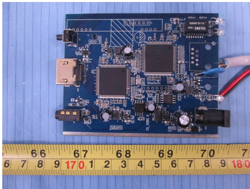
EUT –Main Board 2 Top View (Model: LKV388A)
