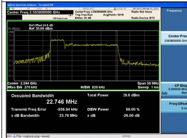
Band41C / 5MHz+20MHz / 64QAM/ Mid CH
