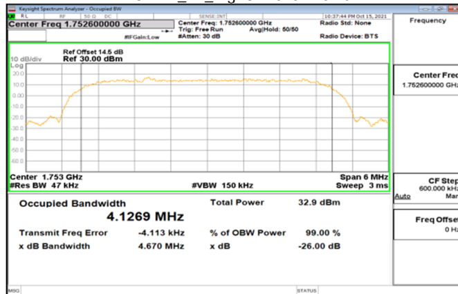
WCDMA_B4_HighCH1513-1752.6
