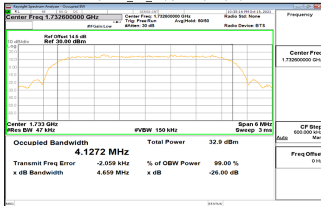
WCDMA_B4_MidCH1413-1732.6
