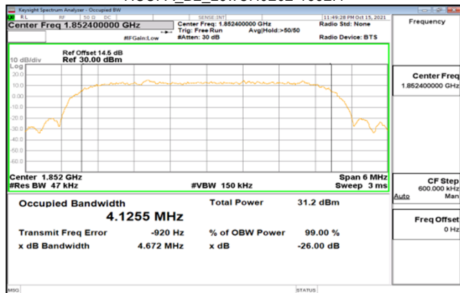
HSUPA_B2_LowCH9262-1852.4
