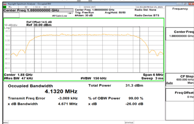
HSUPA_B2_MidCH9400-1880
