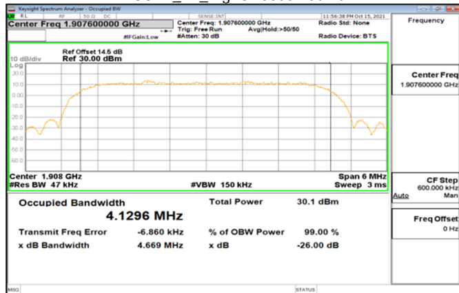
HSUPA_B2_HighCH9538-1907.6
