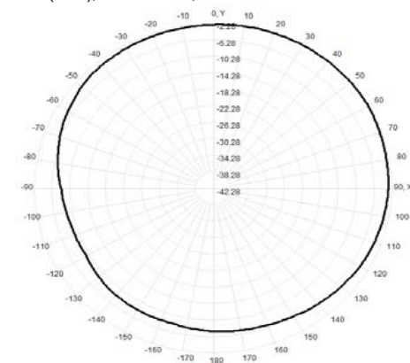
Total(H-XY), Max= -2.28dBi, CirD=7.29
