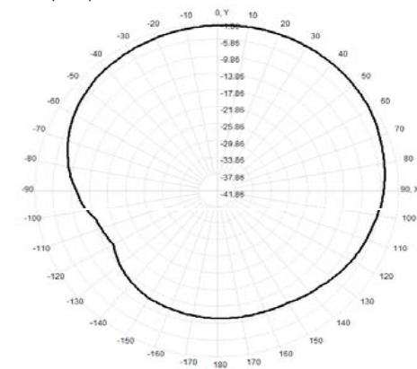
Total(H-XY), Max= -2.23dBi, CirD=13.49
