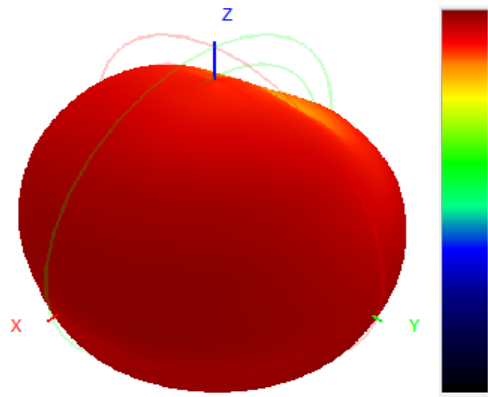
910.0MHz H+V, Eff: 40.6%
