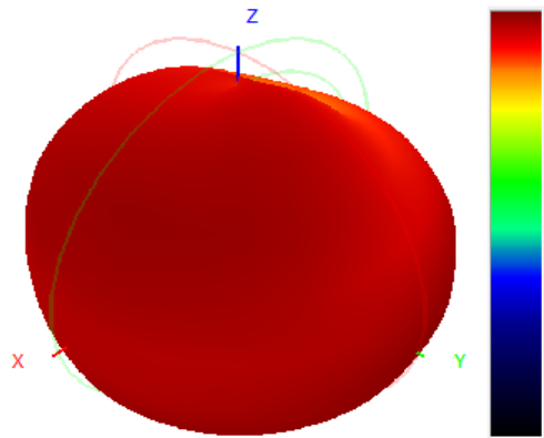
860.0MHz H+V, Eff: 46.5%
