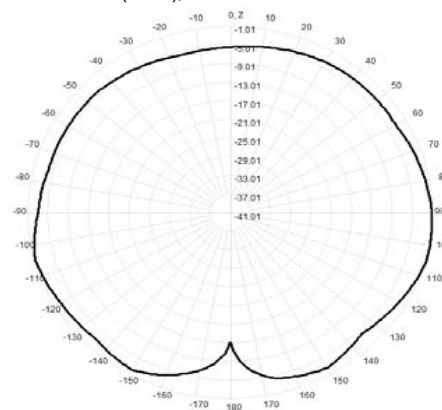
890.0MHz Total(E2-YZ), Max= -1.01dBi
