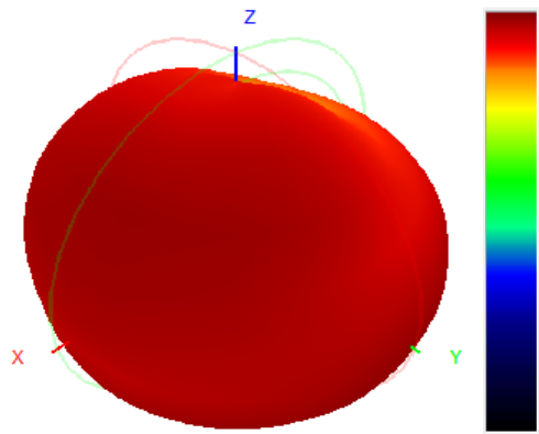
880.0MHz H+V, Eff: 52.3%
