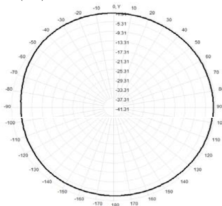
Total(H-XY), Max= -1.60dBi, CirD=3.52
