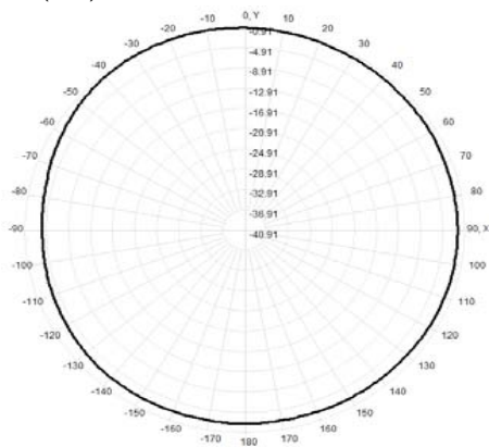
Total(H-XY), Max= -0.93dBi, CirD=3.24
