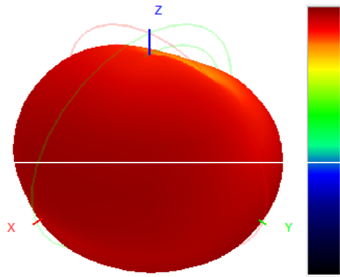
900.0MHz H+V, Eff: 46.4%
