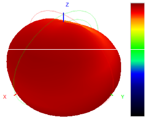
870.0MHz H+V, Eff: 53.0%
