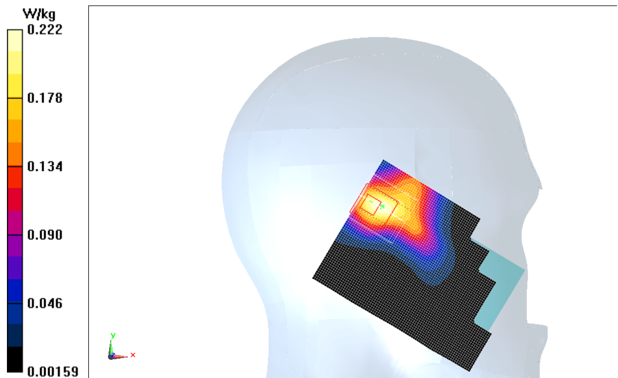
Fig.7 2450 MHz CH11
