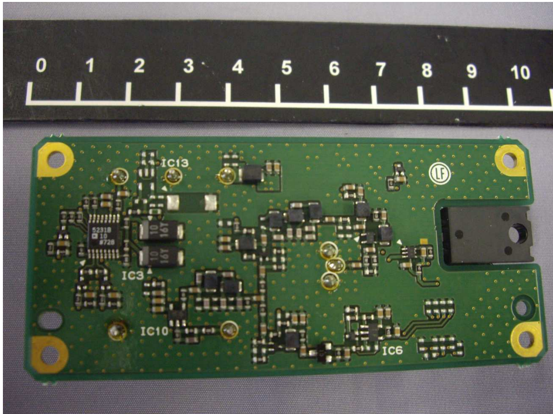
KXK-3 (OCXO) Bottom Side View
