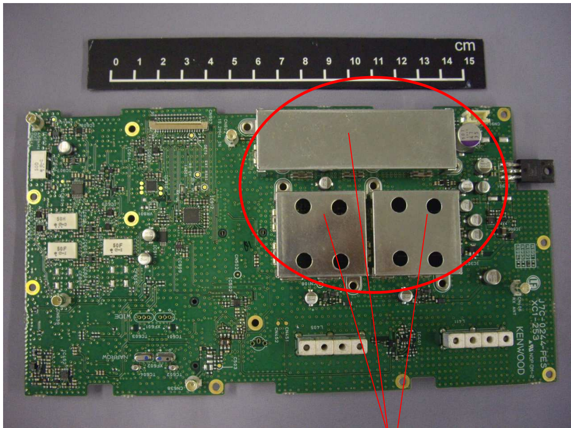
RX UNIT Upper Side View with Shield
