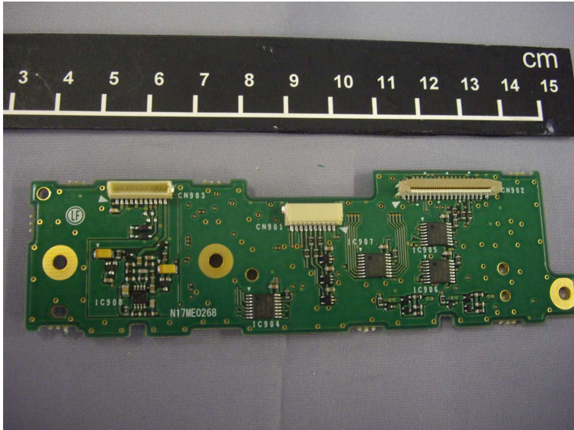
TX UNIT 2 Bottom Side View
