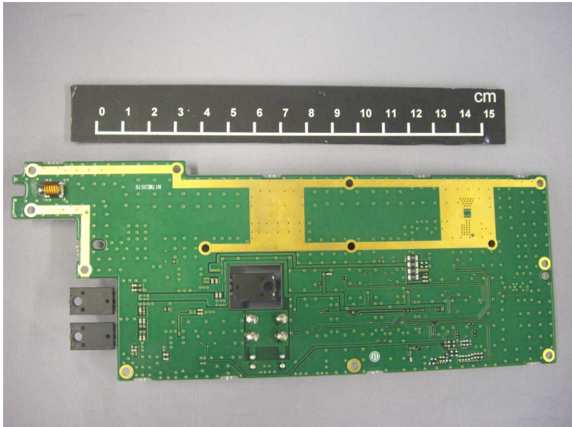
Final Unit 1 Bottom Side View
