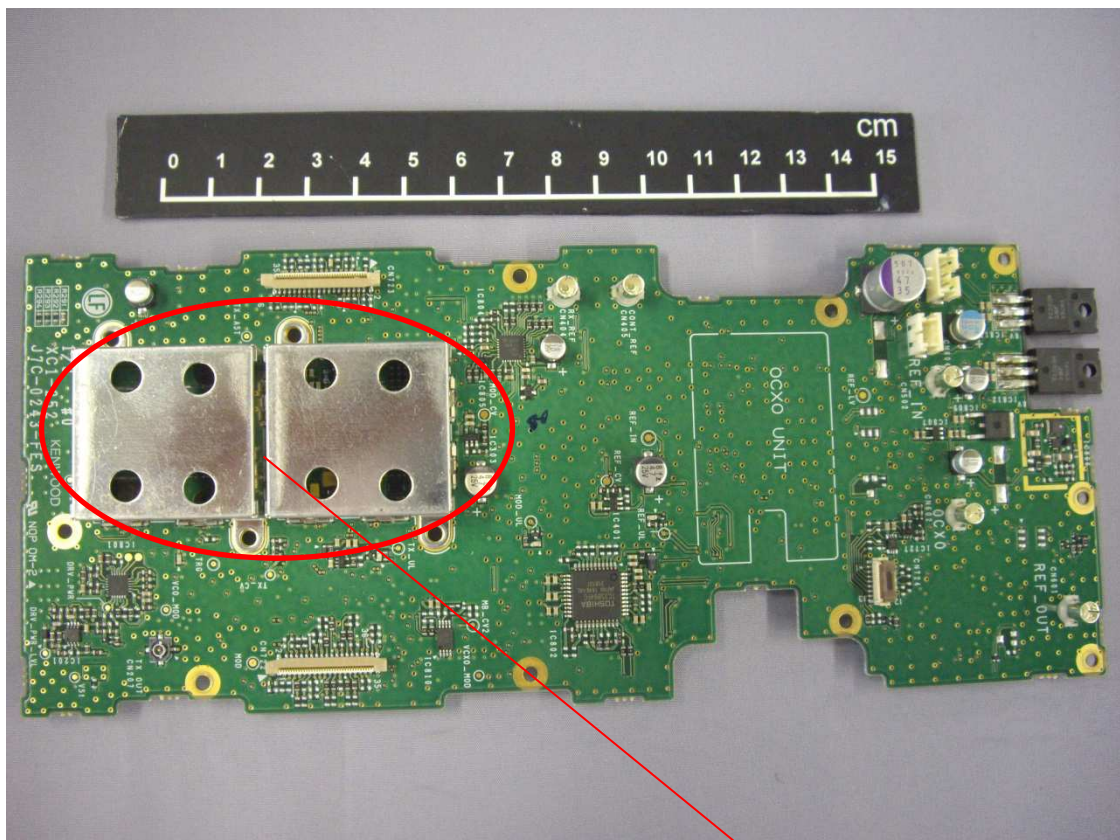
TX UNIT 1 Upper Side View with Shield
