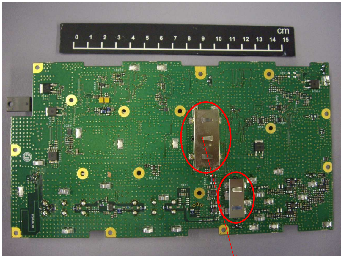
RX UNIT Bottom Side View with Shield
