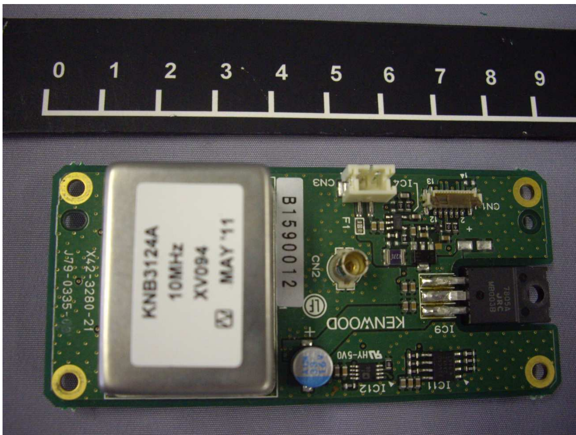
KXK-3 (OCXO) Upper Side View
