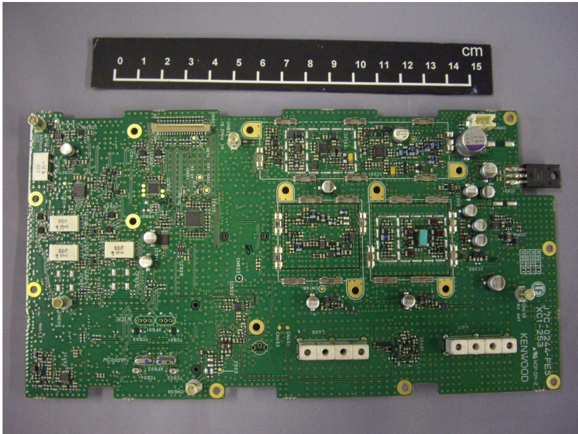
RX UNIT Upper Side View
