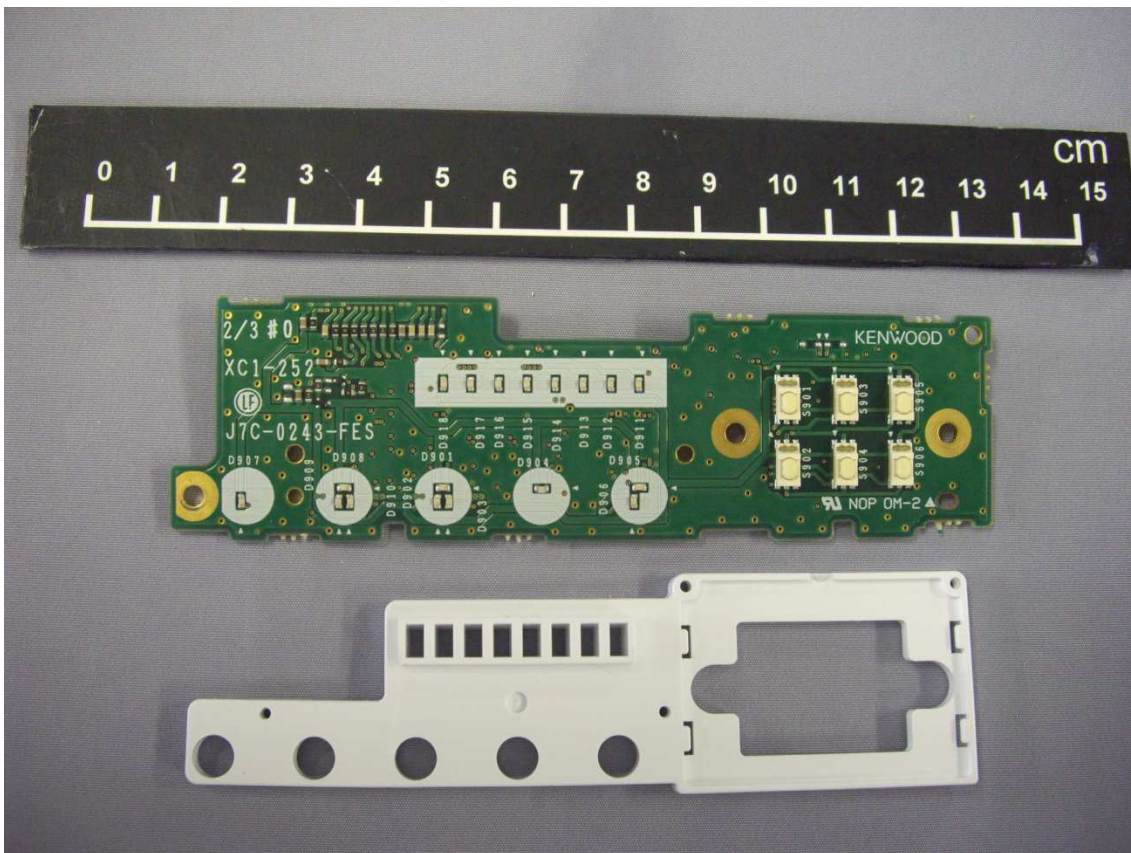
TX UNIT 2 Upper Side View
