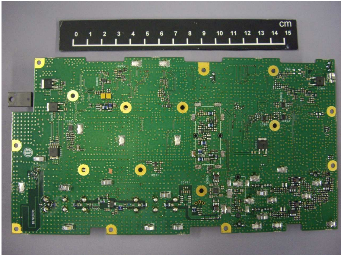
RX UNIT Bottom Side View
