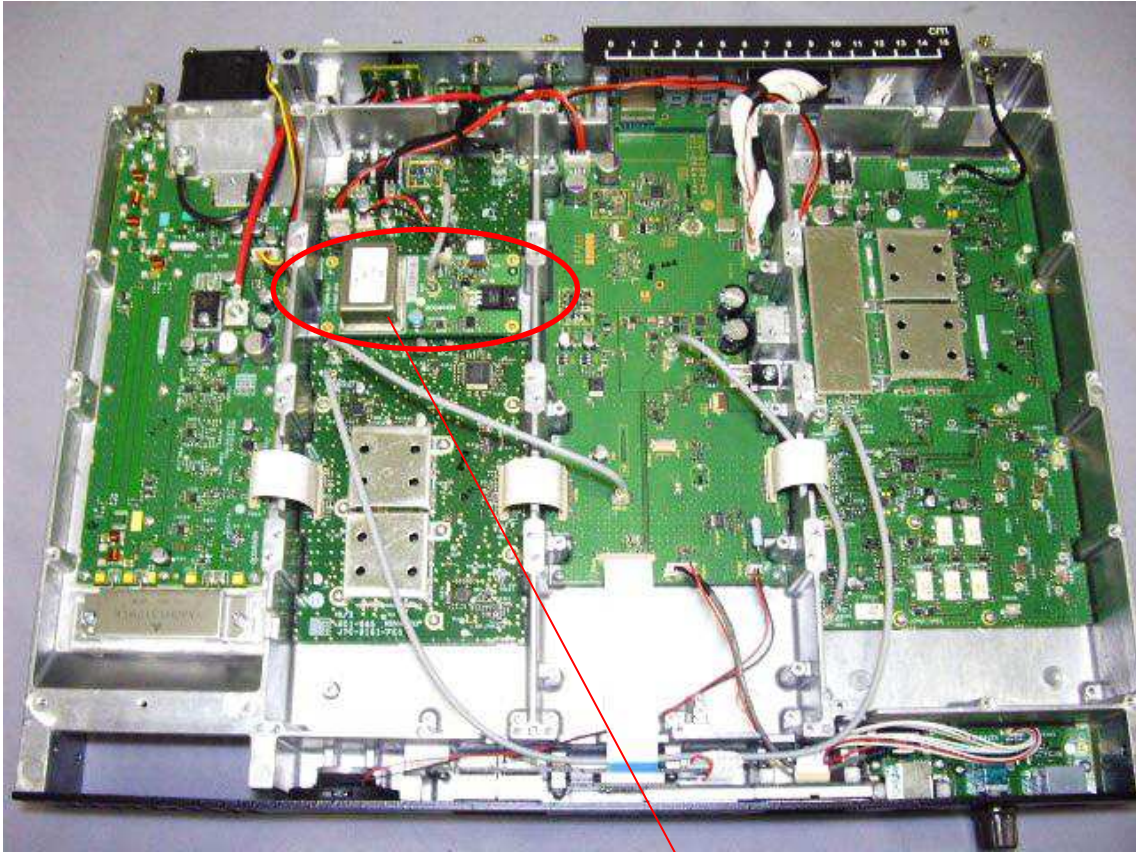
(Upper Side View with KXK-3 (OCXO))
