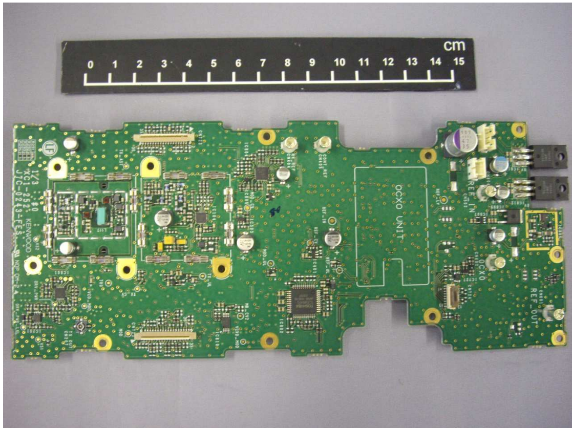
TX UNIT 1 Upper Side View
