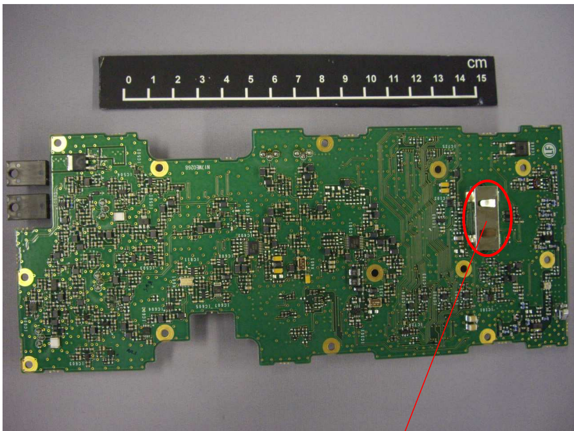
TX UNIT 1 Bottom Side View with Shield
