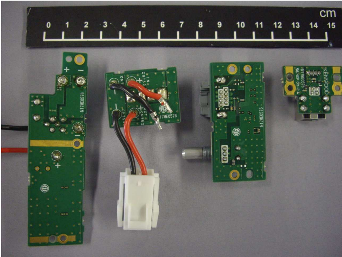
Final Unit 2~5 Bottom Side View
