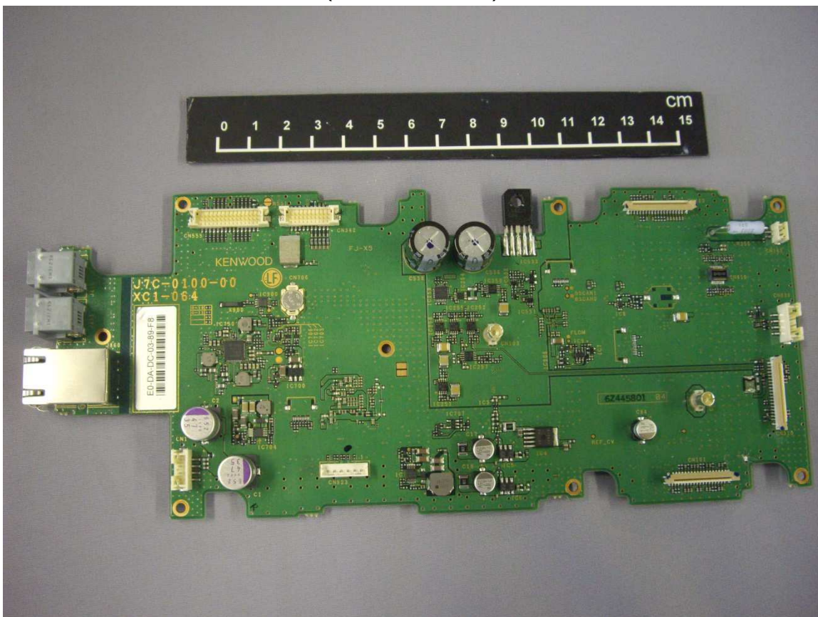
Control UNIT Upper Side View
