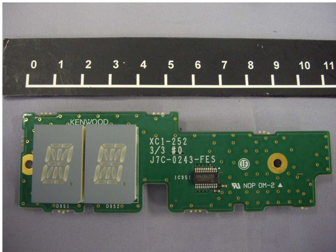
TX UNIT 3 Upper Side View
