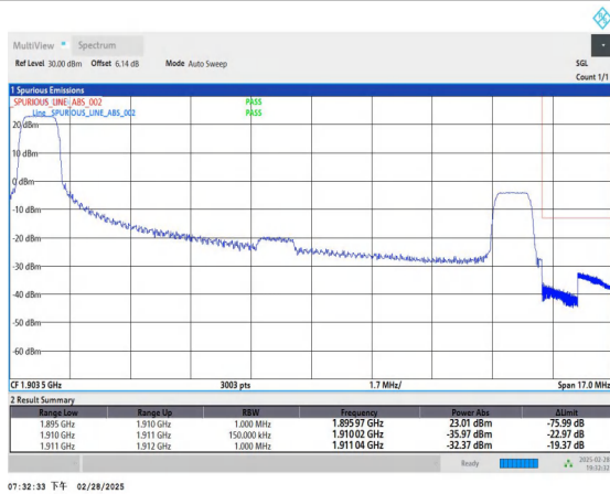
Band2_15MHz_QPSK_19125_1RB#0
