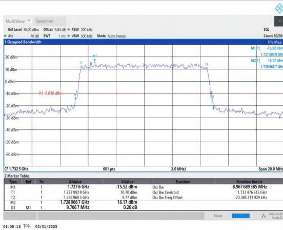
Band4-10MHz-QPSK-20175-50RB#0-PASS
