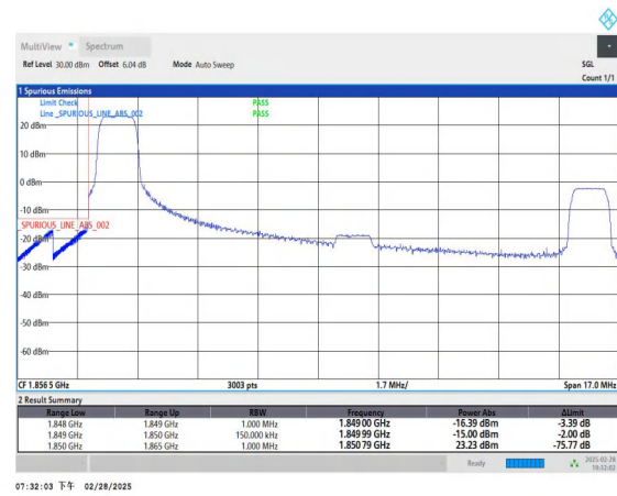
Band2_15MHz_QPSK_18675_1RB#0
