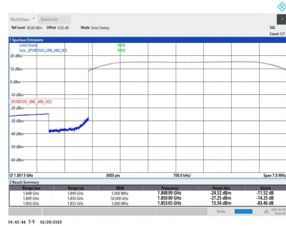
Band2_5MHz_QPSK_18625_25RB#0
