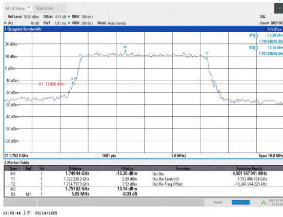
Band4-5MHz-16QAM-20375-25RB#0-PASS
