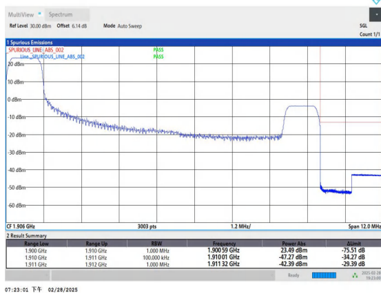
Band2_10MHz_QPSK_19150_1RB#0
