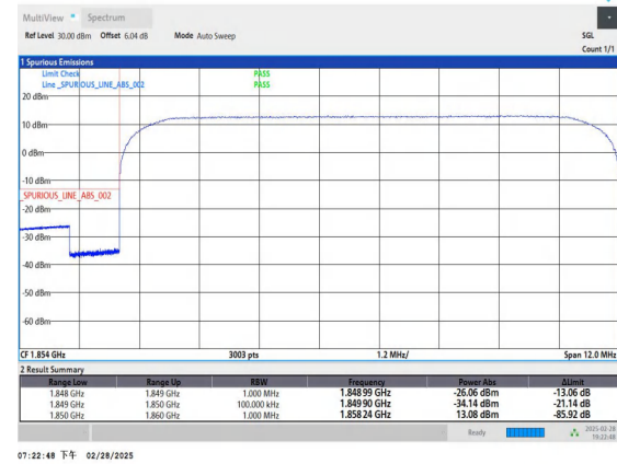
Band2_10MHz_QPSK_18650_50RB#0
