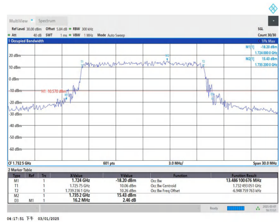
Band4-15MHz-QPSK-20175-75RB#0-PASS
