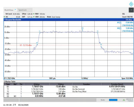
Band4-5MHz-16QAM-20175-25RB#0-PASS
