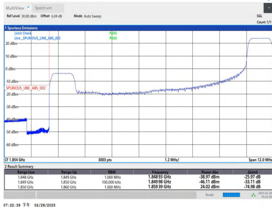
Band2_10MHz_QPSK_18650_1RB#49
