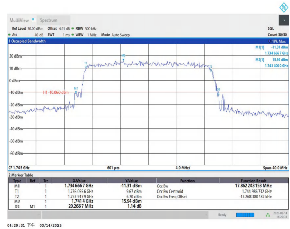
Band4-20MHz-QPSK-20300-100RB#0-PASS
