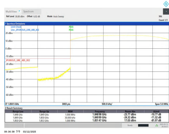
Band2_3MHz_QPSK_18615_15RB#0
