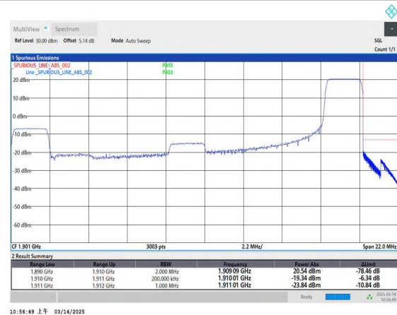
Band2_20MHz_QPSK_19100_1RB#99
