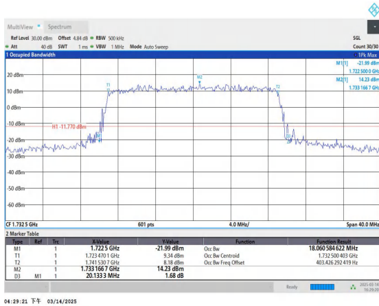
Band4-20MHz-QPSK-20175-100RB#0-PASS
