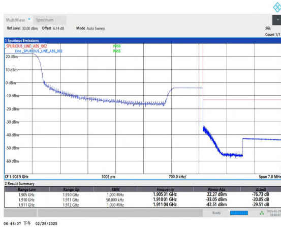
Band2_5MHz_QPSK_19175_1RB#0
