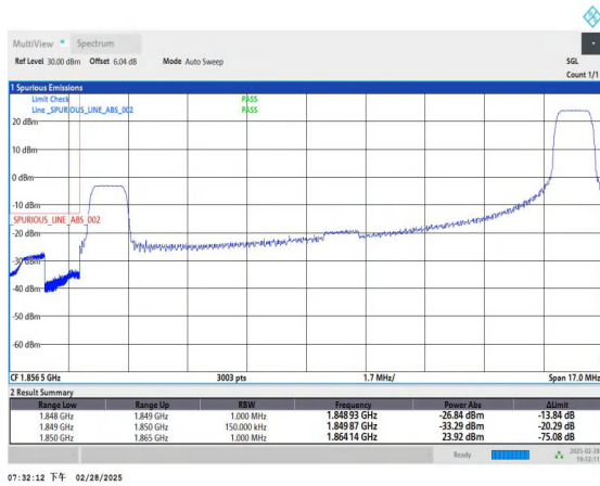
Band2_15MHz_QPSK_18675_1RB#74
