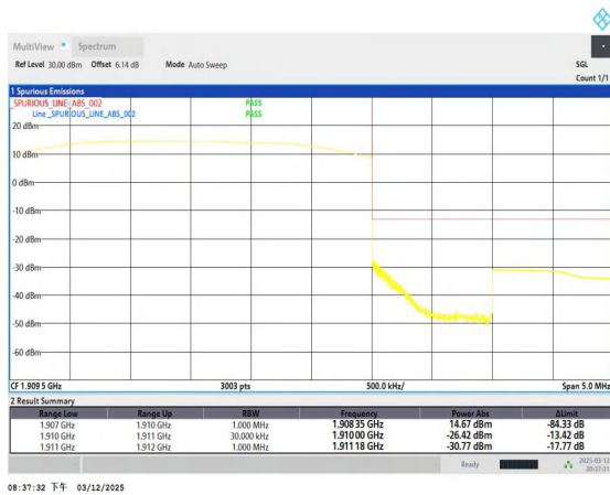
Band2_3MHz_QPSK_19185_15RB#0
