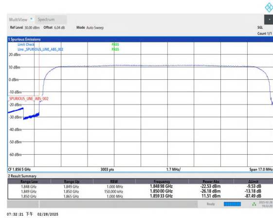
Band2_15MHz_QPSK_18675_75RB#0
