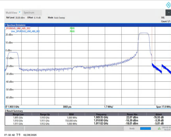
Band2_15MHz_QPSK_19125_1RB#74
