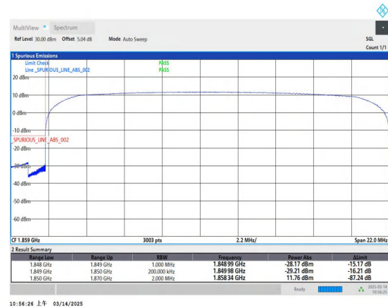
Band2_20MHz_QPSK_18700_100RB#0
