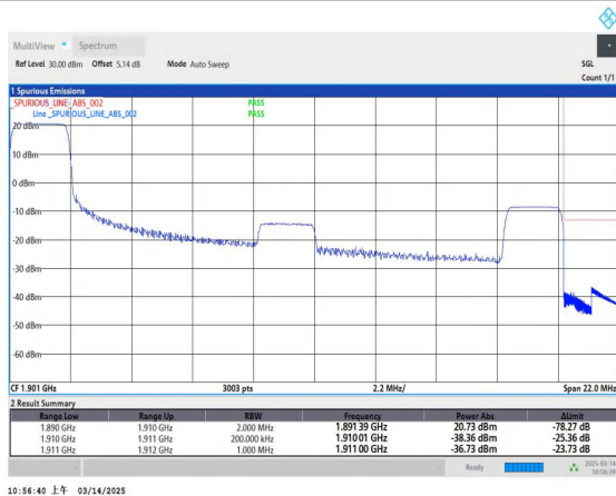
Band2_20MHz_QPSK_19100_1RB#0
