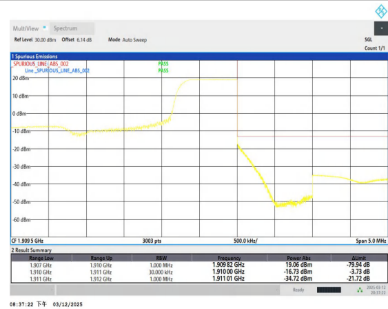
Band2_3MHz_QPSK_19185_1RB#14
