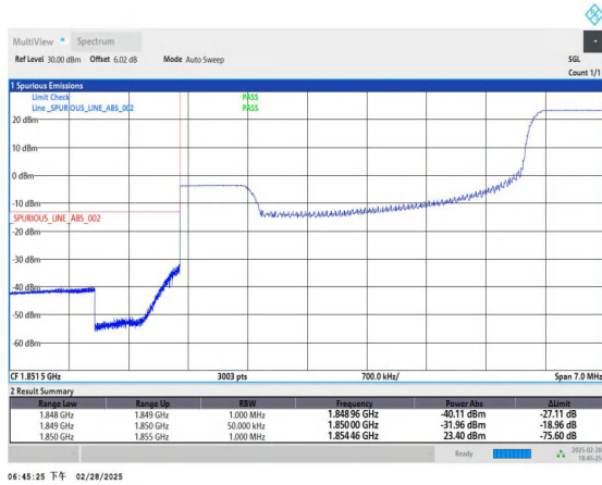
Band2_5MHz_QPSK_18625_1RB#24
