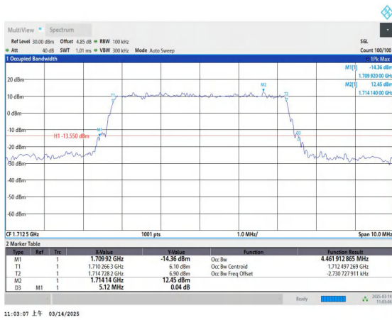
Band4-5MHz-16QAM-19975-25RB#0-PASS
