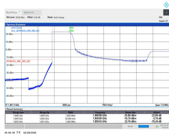
Band2_5MHz_QPSK_18625_1RB#0
