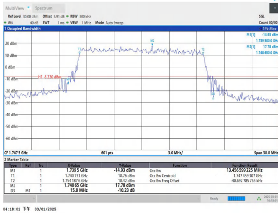
Band4-15MHz-QPSK-20325-75RB#0-PASS
