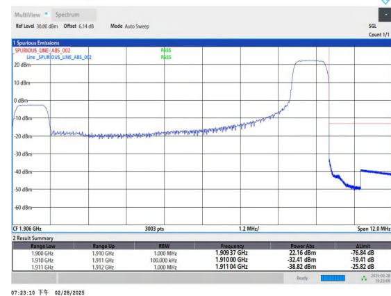
Band2_10MHz_QPSK_19150_1RB#49
