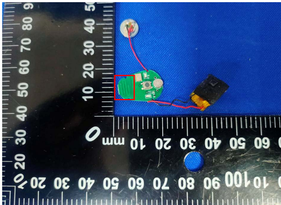
BT Antenna
