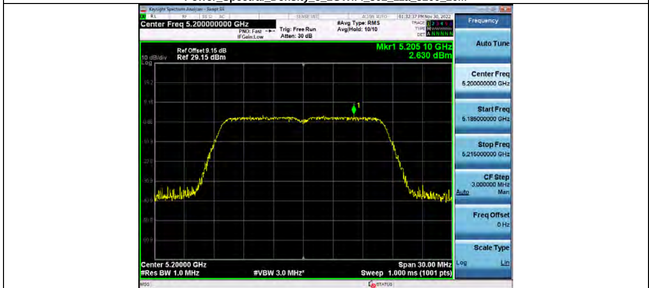
Power_Spectral_Density_5_2GWiFi_802_11a_5200_20M
