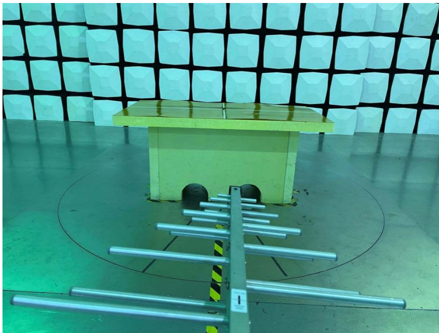
Below 1GHz(BT)
