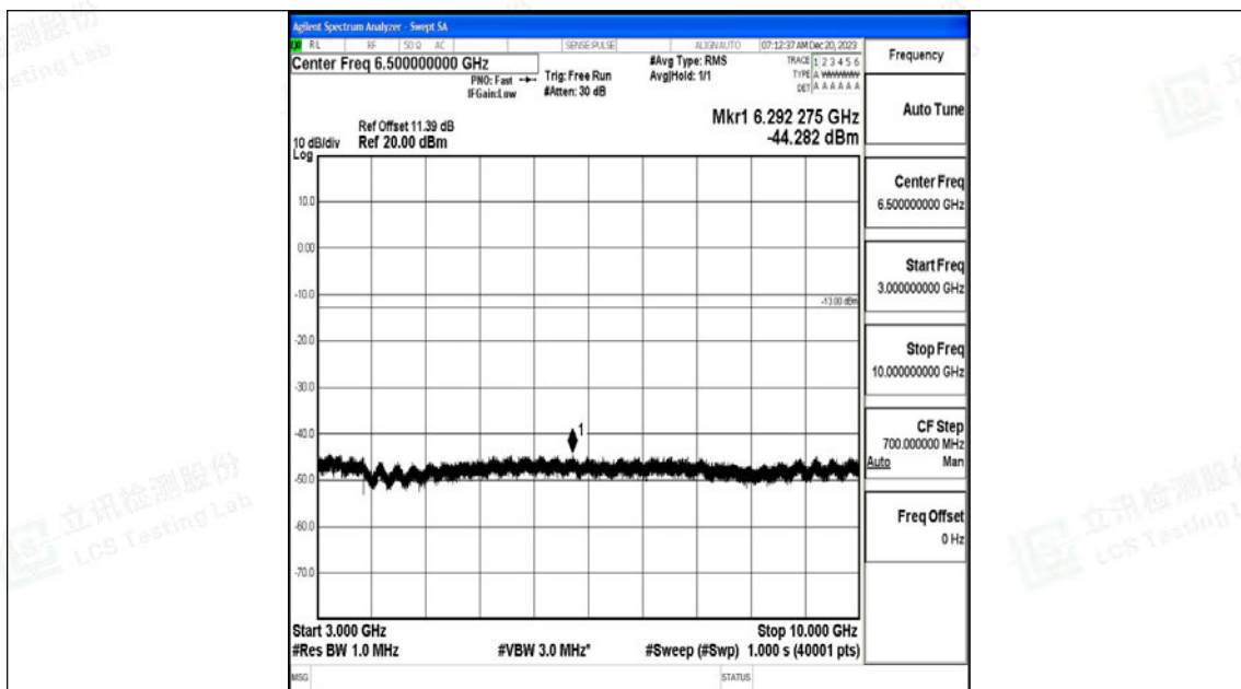
Band5_5MHz_QPSK_20625_1RB#0_3000~10000_3000~10000
