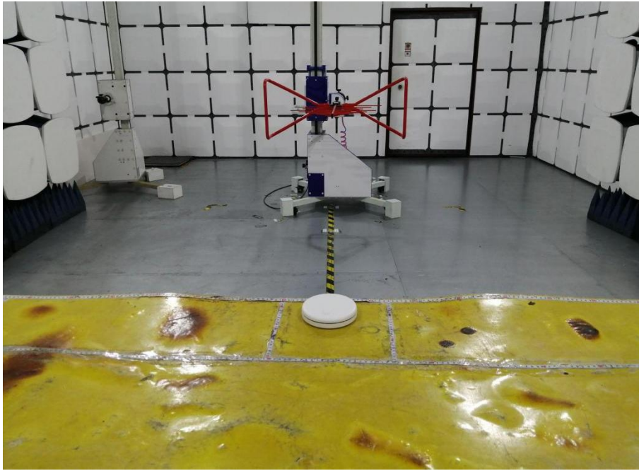
Emissions in frequency bands (below 1GHz)
