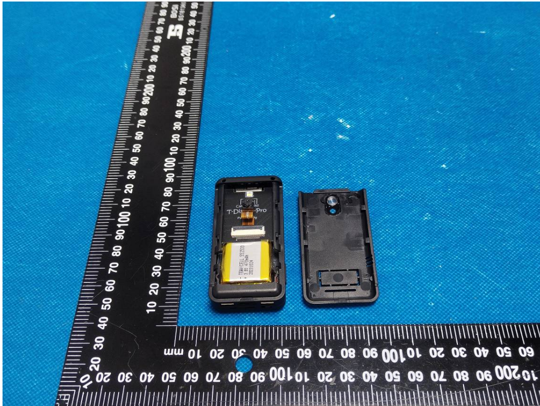
T-Display-S3 Pro (Black Shell GC0308 Camera)
