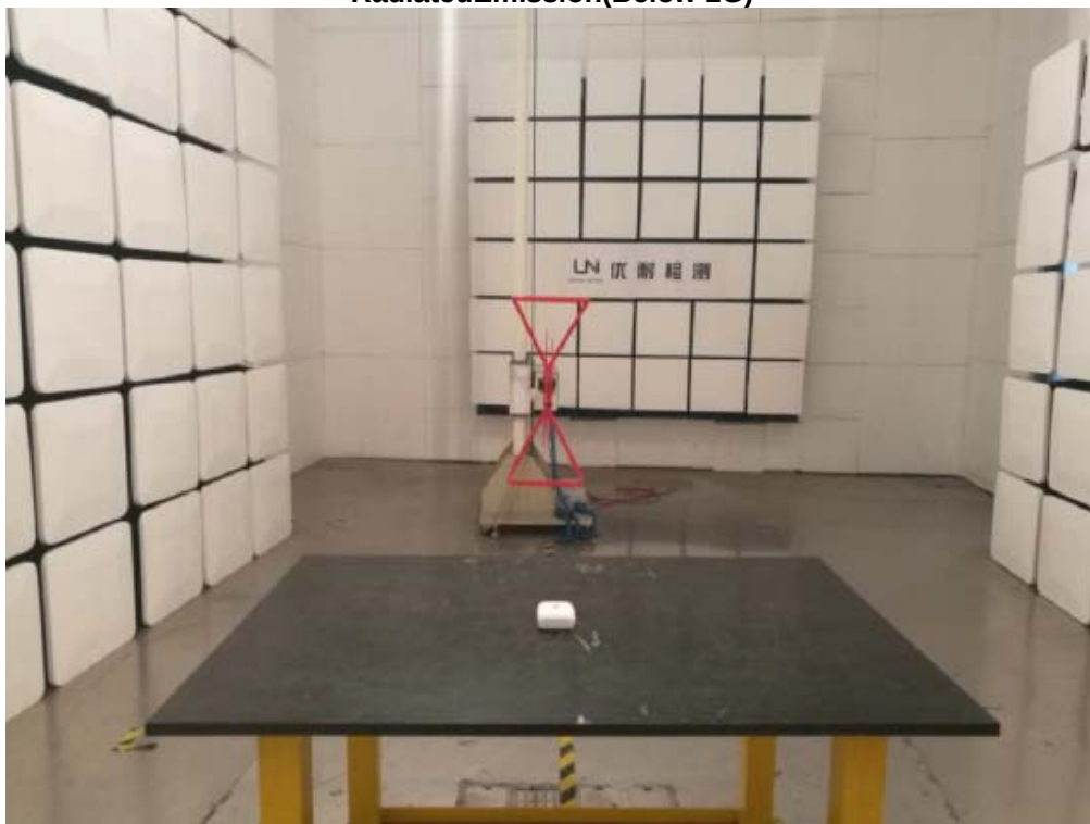
RadiatedEmission(Below 1G)
