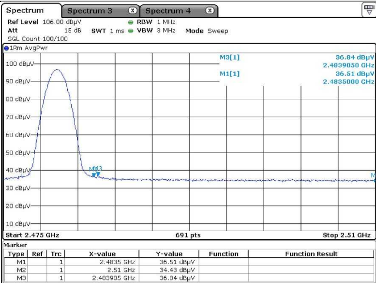
Radiated restricted band edge plot - 2 480 MHz (Average)
