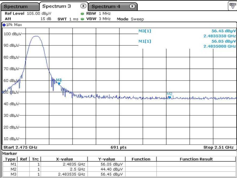
Radiated restricted band edge plot - 2 480 MHz (Peak)
