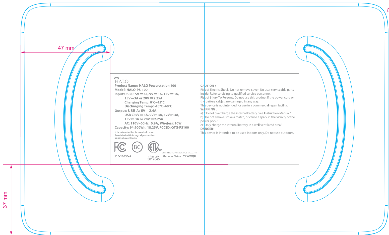
bottom view
