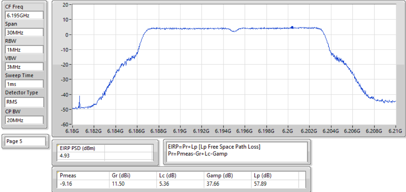
EIRP PSD;Band:6.2G;11a;BWch:20MHz;Nss:1,(6D);Nant:1(1);Ch:6195MHz;TX
