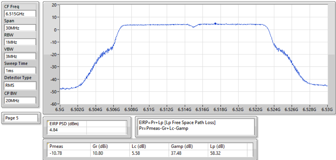
EIRP PSD;Band:6.4G;11a;BWch:20MHz;Nss:1,(6D);Nant:1(1);Ch:6515MHz;TX
