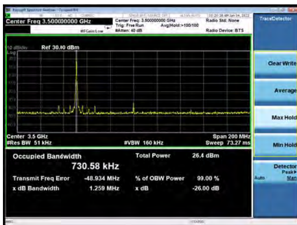
NR n77 Subset 1 16QAM 1RB 100MHz CH- Middle
