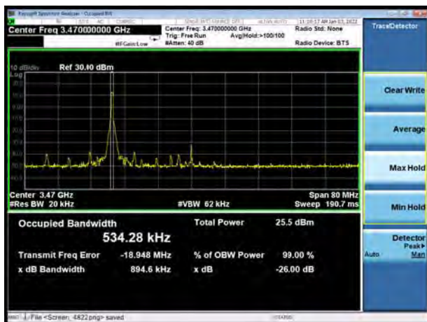
NR n77 Subset 1 64QAM 1RB 40MHz CH-Middle
