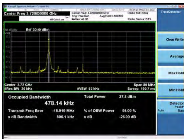
DC_66A_n78 P1/2 BPSK 1RB 40MHz CH-Middle
