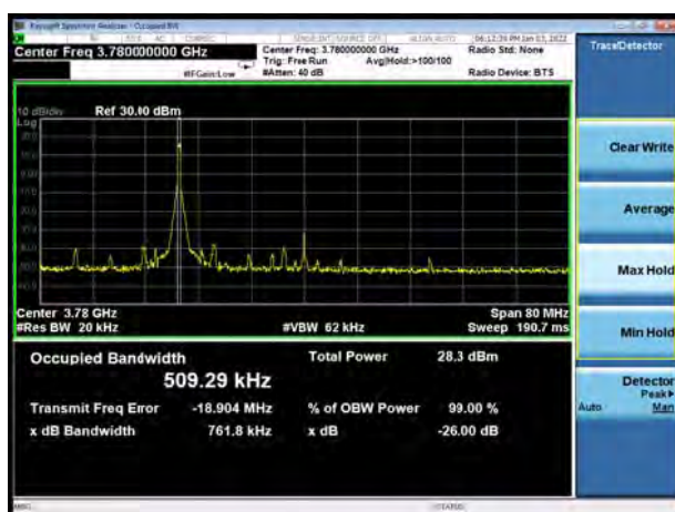
DC_66A_n78 P1/2 BPSK 1RB 40MHz CH-High
