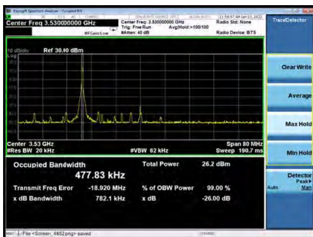
NR n77 Subset 1 64QAM 1RB 40MHz CH-High
