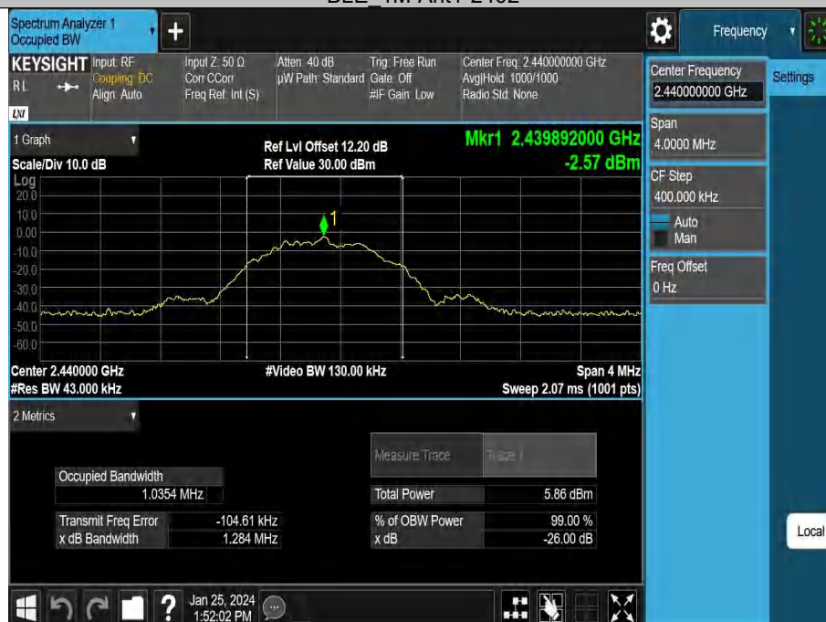
BLE_1M-Ant1-2440
