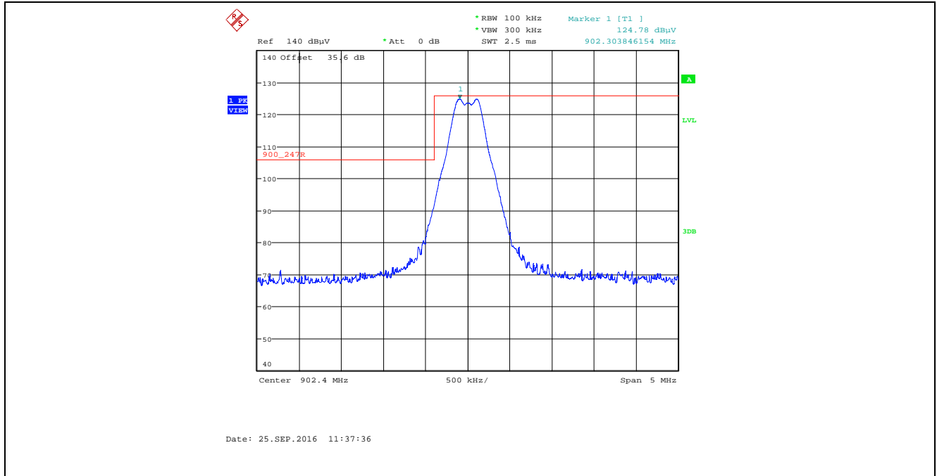
Plot 5.2.4.2.2.1. Band-Edge RF Radiated Emissions at 3 m, Horizontal Polarization Single Frequency Mode, Low End of Frequency Band, Power Setting 28, Data Rate at 276480 kbps
