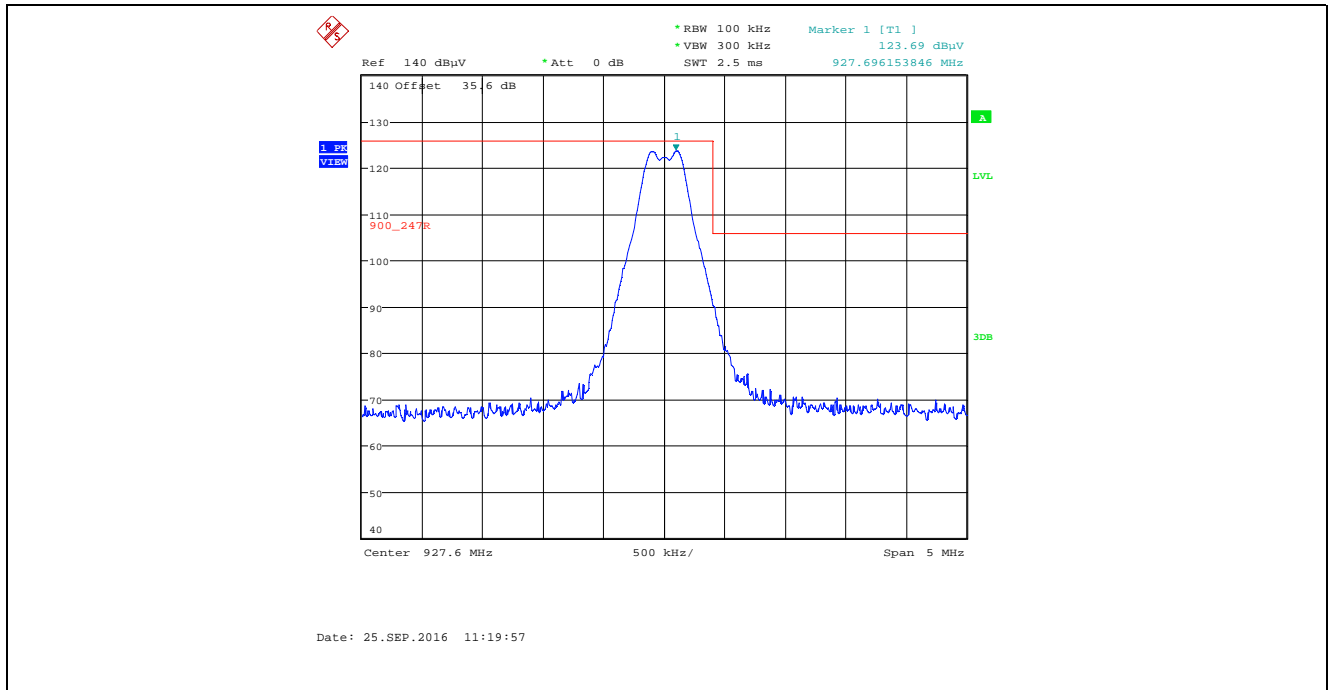
Plot 5.2.4.2.2.7. Band-Edge RF Radiated Emissions at 3 m, Vertical Polarization Single Frequency Mode, High of Frequency Band, Power Setting 28, Data Rate at 276480 kbps
