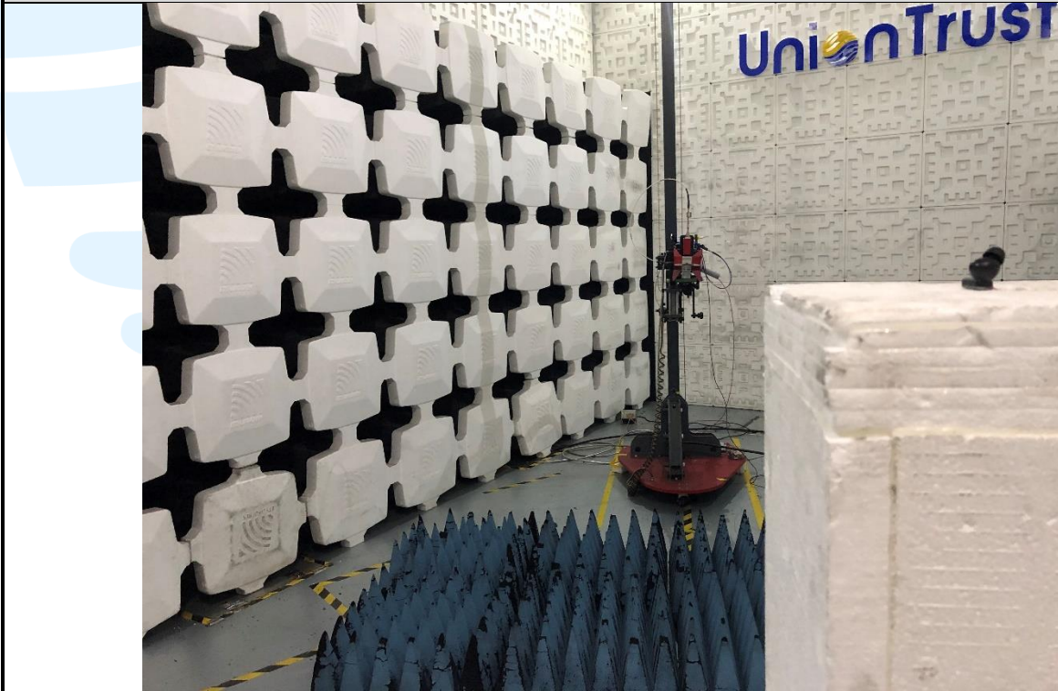
Radiated emission Test Setup (Above 1 GHz) -Right
