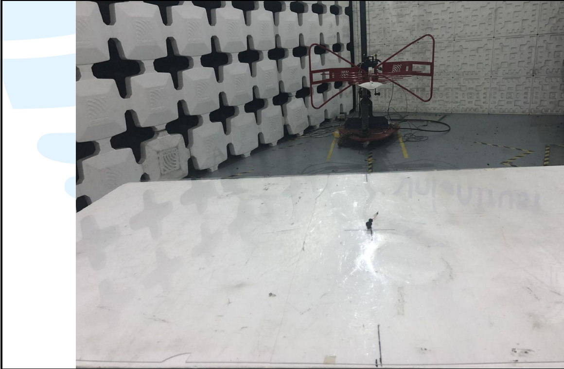
Radiated emission Test Setup (30 MHz~1 GHz) -Right
