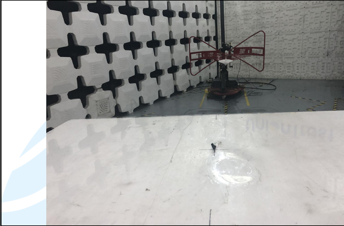
Radiated emission Test Setup (30 MHz~1 GHz) -Left
