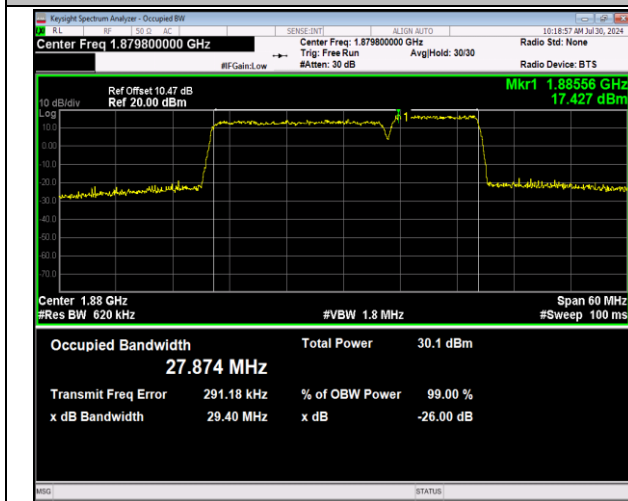
2-2-20MHz-10MHz-64QAM-64QAM-18851-18995-100RB#0-50RB#0-PASS
