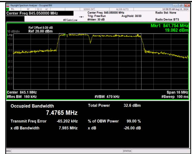
5-5-3MHz-5MHz-16QAM-16QAM-20586-20625-15RB#0-2 5RB#0-PASS
