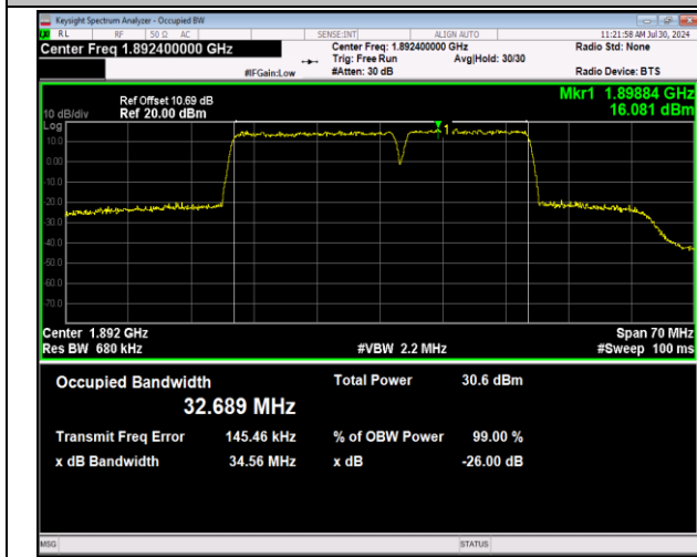
2-2-20MHz-15MHz-64QAM-64QAM-18951-19122-100RB#0-75RB#0-PASS
