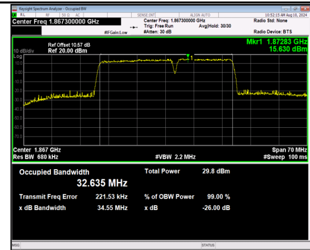
2-2-20MHz-15MHz-16QAM-16QAM-18700-18871-100RB#0-75RB#0-PASS
