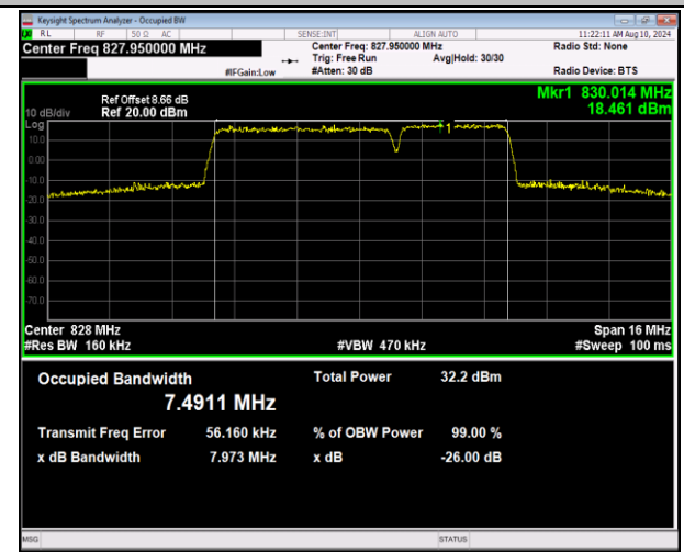
5-5-5MHz-3MHz-QPSK-QPSK-20425-20464-25RB#0-15R B#0-PASS
