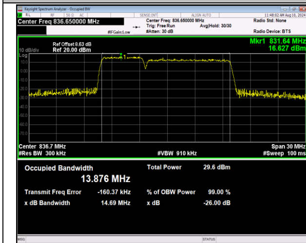
5-5-5MHz-10MHz-16QAM-16QAM-20478-20550-25RB#0-50 50RB#0-PASS
