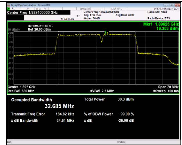
2-2-20MHz-15MHz-16QAM-16QAM-18951-19122-100RB#0-75RB#0-PASS
