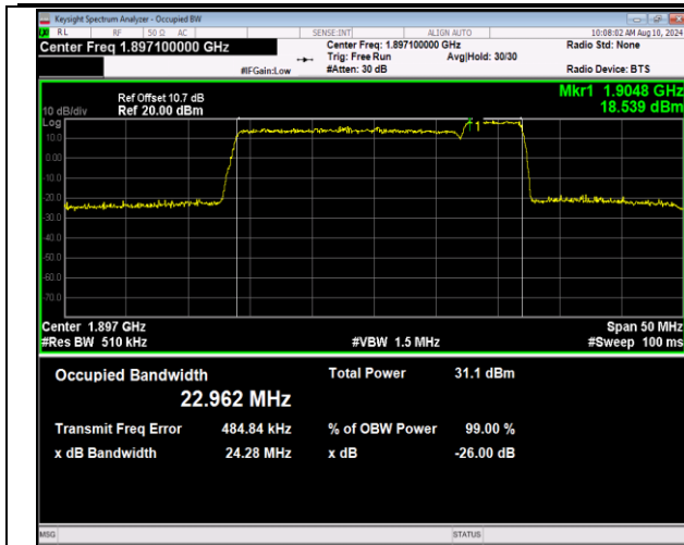
2-2-20MHz-5MHz-QPSK-QPSK-19050-19167-100RB#0-2 5RB#0-PASS
