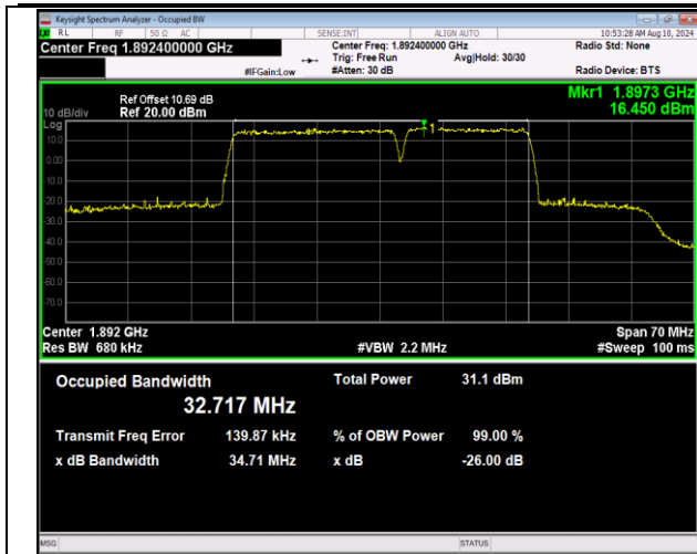
2-2-20MHz-15MHz-QPSK-QPSK-18951-19122-100RB#0-75RB#0-PASS
