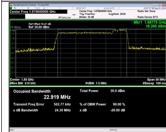
2-2-20MHz-5MHz-16QAM-16QAM-18875-18992-100RB#0-2 -25RB#0-PASS
