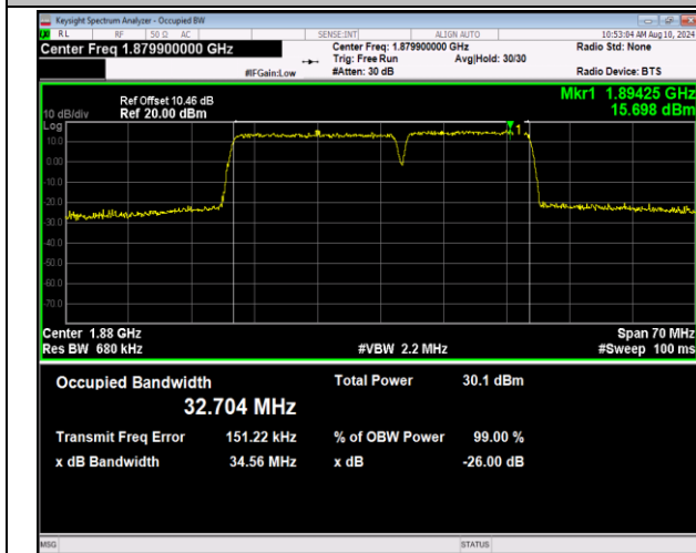
2-2-20MHz-15MHz-16QAM-16QAM-18826-18997-100RB#0-75RB#0-PASS
