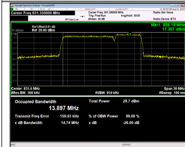
5-5-10MHz-5MHz-16QAM-16QAM-20450-20522-50RB#0-25RB#0-PASS
