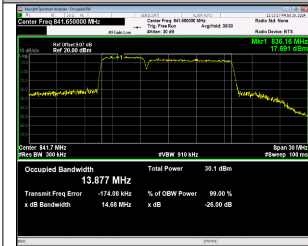
5-5-5MHz-10MHz-64QAM-64QAM-20528-20600-25RB#0-50RB#0-PASS
