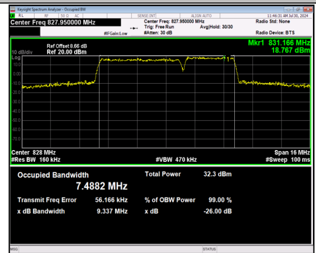
5-5-5MHz-3MHz-64QAM-64QAM-20425-20464-25RB#0-1 5RB#0-PASS
