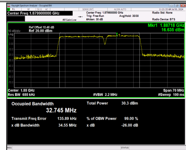
2-2-20MHz-15MHz-64QAM-64QAM-18826-18997-100RB#0-75RB#0-PASS
