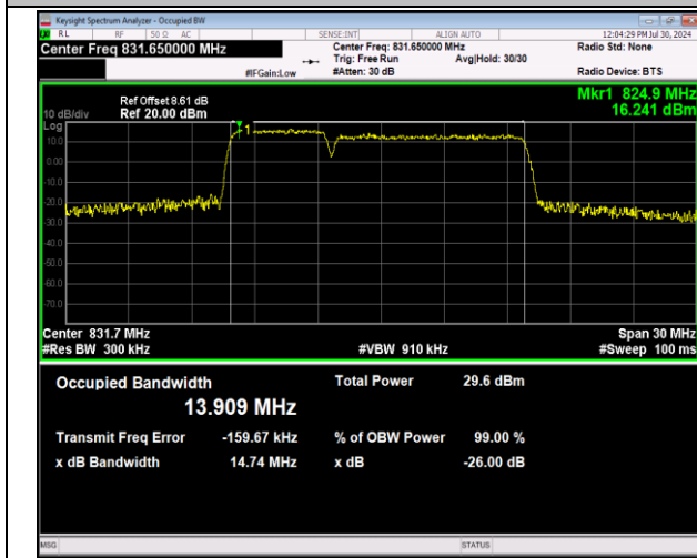
5-5-5MHz-10MHz-64QAM-64QAM-20428-20500-25RB#0-50 50RB#0-PASS
