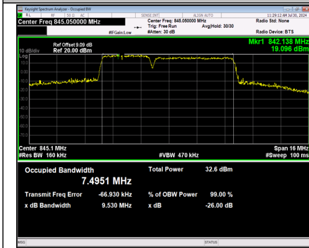
5-5-3MHz-5MHz-64QAM-64QAM-20586-20625-15RB#0-2 5RB#0-PASS
