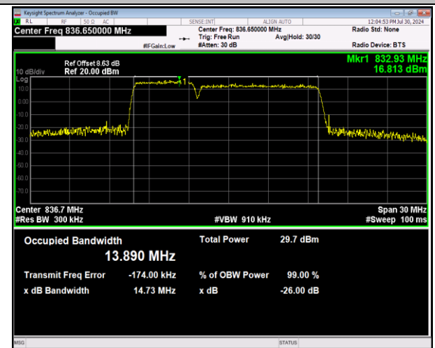
5-5-5MHz-10MHz-64QAM-64QAM-20478-20550-25RB#0-50 50RB#0-PASS
