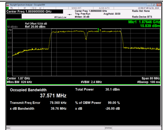
2-2-20MHz-20MHz-64QAM-64QAM-18700-18898-100RB#0-100RB#0-PASS
