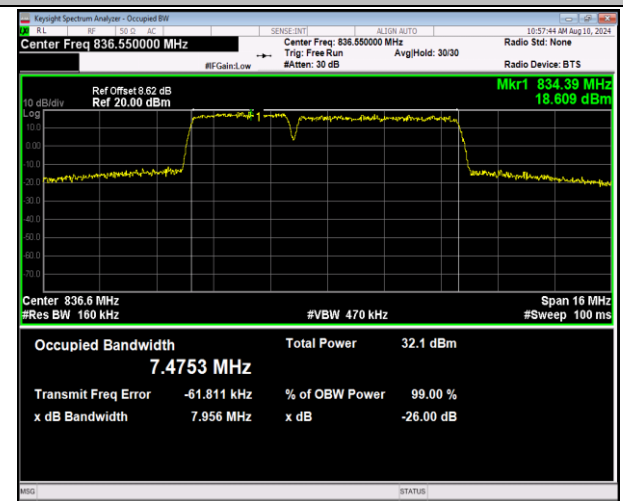
5-5-3MHz-5MHz-QPSK-QPSK-20501-20540-15RB#0-25R B#0-PASS
