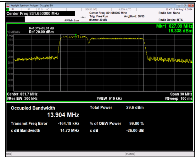
5-5-5MHz-10MHz-16QAM-16QAM-20428-20500-25RB#0-50 50RB#0-PASS
