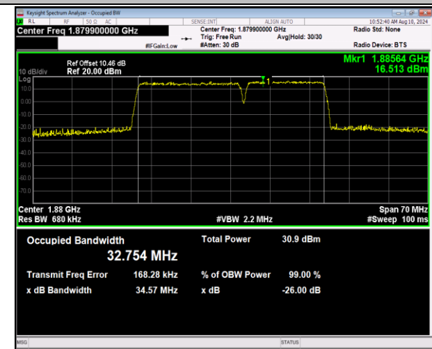
2-2-20MHz-15MHz-QPSK-QPSK-18826-18997-100RB#0-75RB#0-PASS
