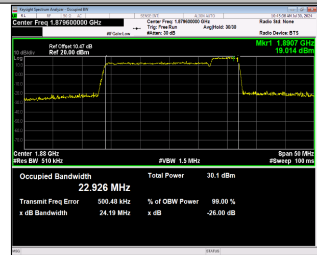
2-2-20MHz-5MHz-64QAM-64QAM-18875-18992-100RB#0-2 -25RB#0-PASS
