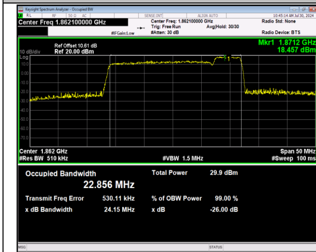
2-2-20MHz-5MHz-64QAM-64QAM-18700-18817-100RB#0-2 -25RB#0-PASS
