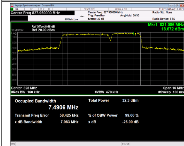
5-5-5MHz-3MHz-16QAM-16QAM-20425-20464-25RB#0-1 5RB#0-PASS
