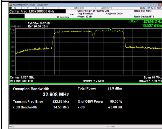
2-2-20MHz-15MHz-64QAM-64QAM-18700-18871-100RB#0-75RB#0-PASS
