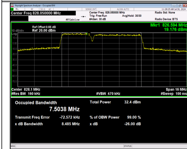
5-5-3MHz-5MHz-64QAM-64QAM-20416-20455-15RB#0-2 5RB#0-PASS
