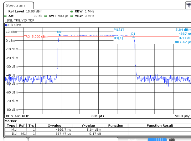
GFSK DH1
