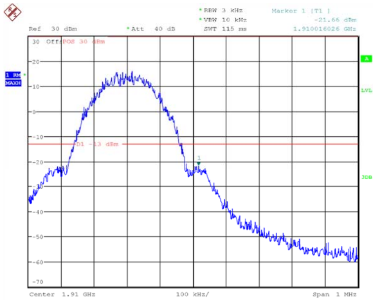
Channel 810- HIGH BAND EDGE BLOCK
