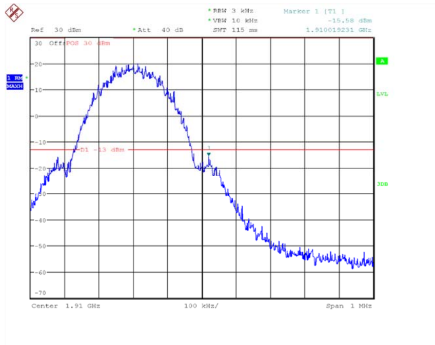
Channel 810- HIGH BAND EDGE BLOCK
