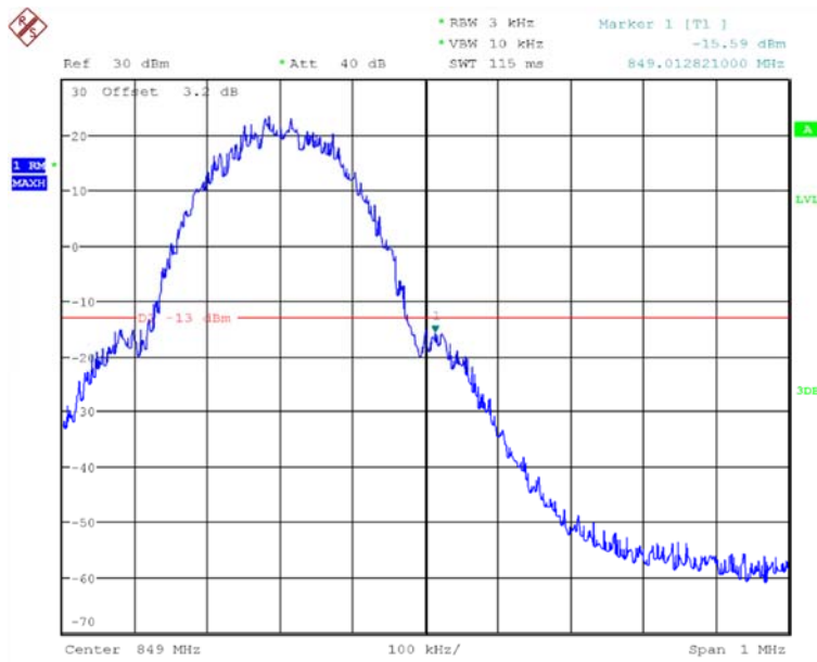
Channel 251- HIGH BAND EDGE BLOCK
