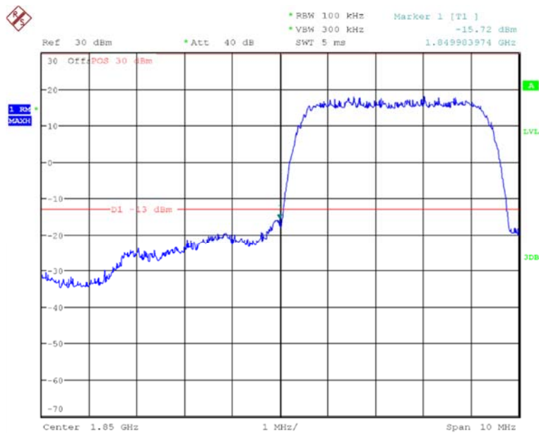
Channel 9262- LOW BAND EDGE BLOCK
