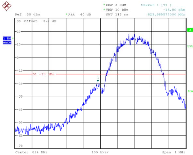
Channel 128- LOW BAND EDGE BLOCK
