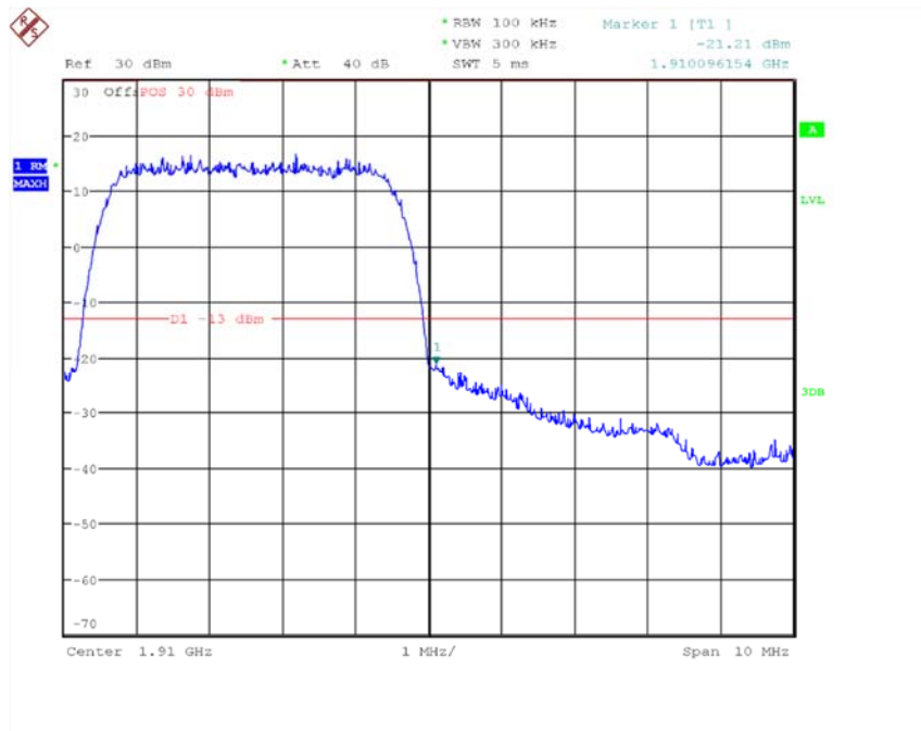
Channel 9538- HIGH BAND EDGE BLOCK
