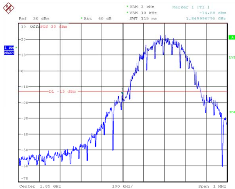
Channel 512- LOW BAND EDGE BLOCK
