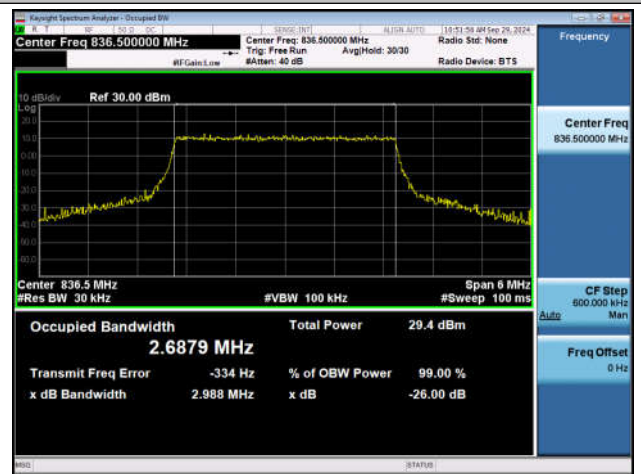
Band5-3MHz-16QAM-20525-15RB#0-PASS
