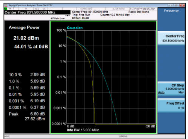
Band26(824-849)-15MHz-16QAM-26865-75RB#0-PASS
