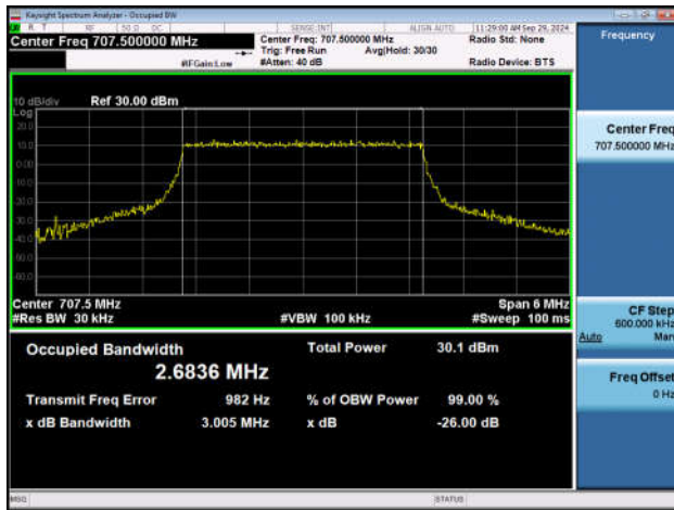
Band12-3MHz-QPSK-23095-15RB#0-PASS
