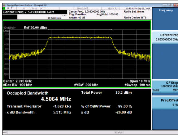
Band41-5MHz-QPSK-40620-25RB#0-PASS
