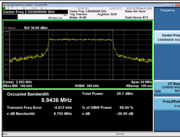
Band41-10MHz-QPSK-40620-50RB#0-PASS
