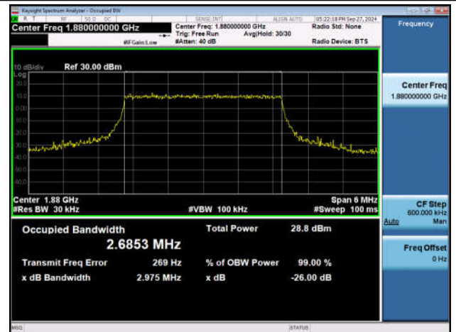
Band2-3MHz-16QAM-18900-15RB#0-PASS
