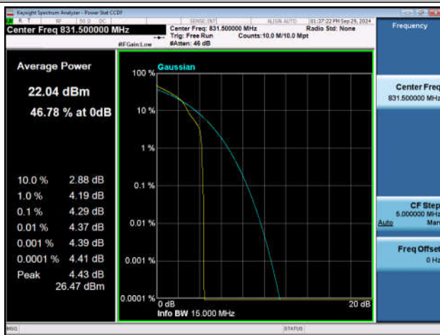
Band26(824-849)-15MHz-16QAM-26865-1RB#0-PASS
