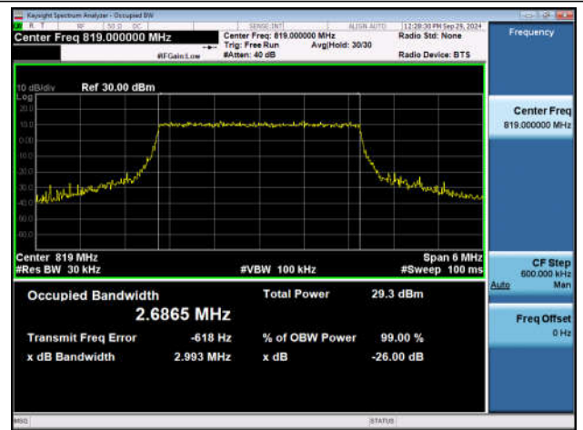
Band26(814-824)-3MHz-16QAM-26740-15RB#0-PASS
