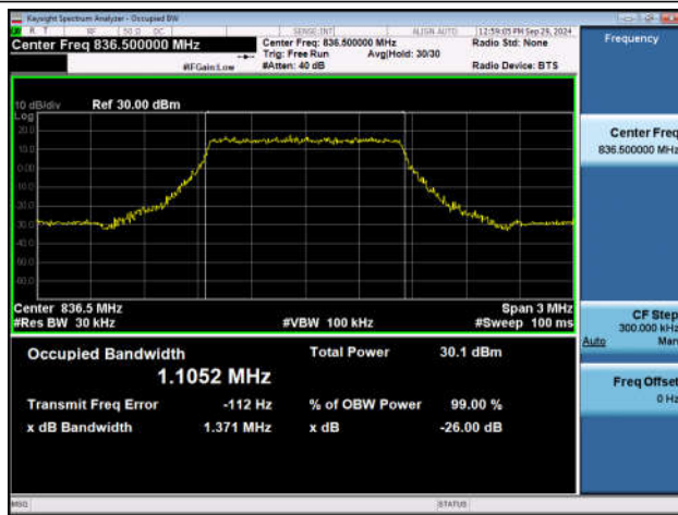
Band26(824-849)-1.4MHz-QPSK-26915-6RB#0-PASS
