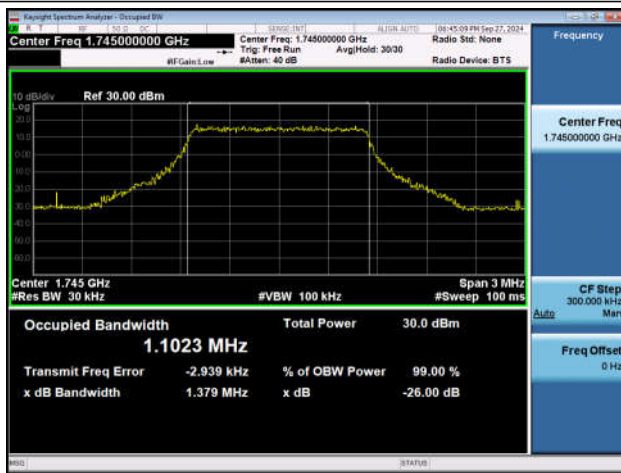
Band66-1.4MHz-QPSK-132322-6RB#0-PASS
