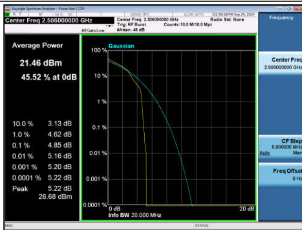
Band41-20MHz-16QAM-39750-1RB#0-PASS
