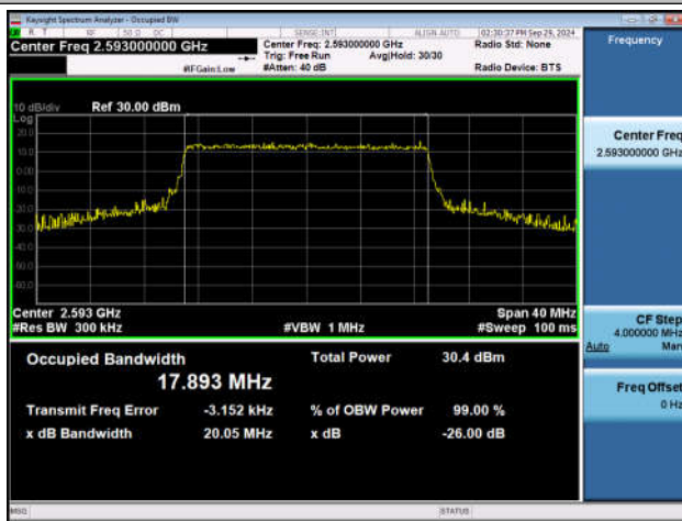
Band41-20MHz-QPSK-40620-100RB#0-PASS
