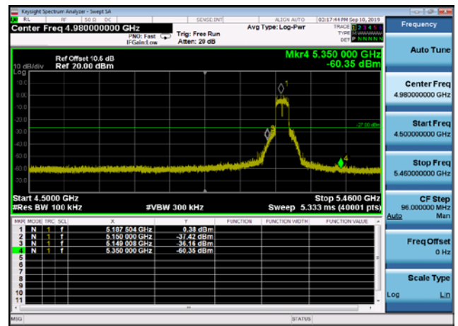
U-NII-1 Band Edge-802.11a(20MHz) ,5180MHz
