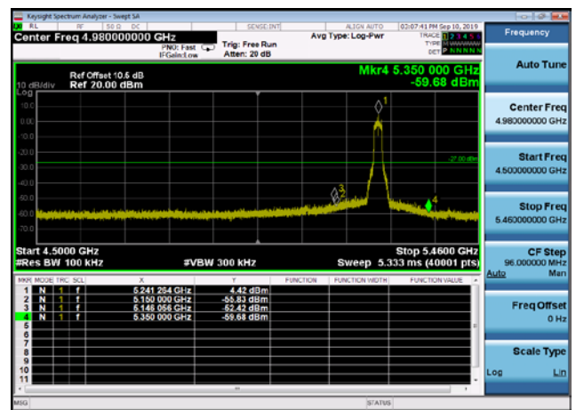
U-NII-1 Band Edge-802.11a(20MHz) ,5240MHz
