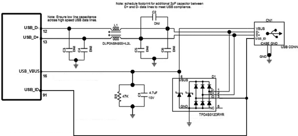
Figure 4-3: USB Interface
