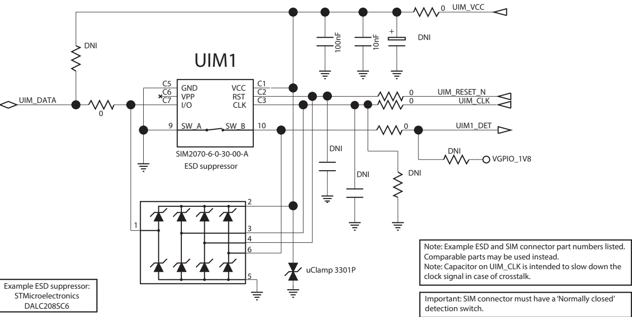
Figure 4-2: UIM Interface
