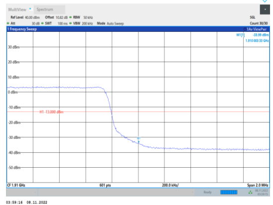
Band2-5MHz-QPSK-19175-25RB#0
