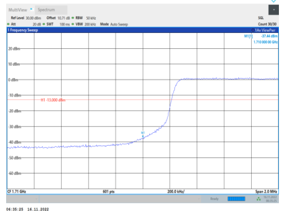
Band4-5MHz-64QAM-19975-25RB#0
