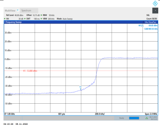
Band2-5MHz-16QAM-18625-25RB#0
