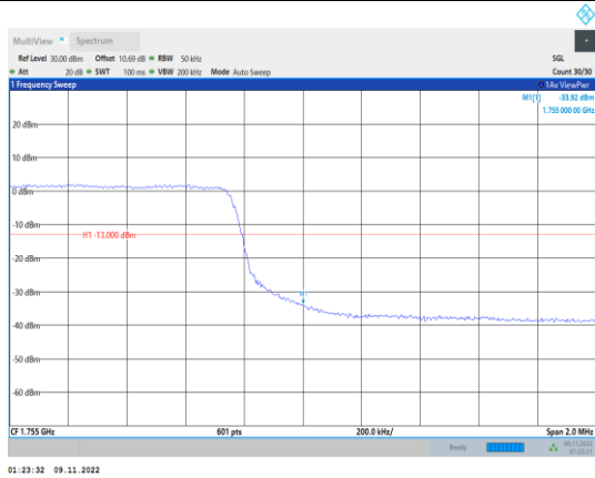
Band4-5MHz-16QAM-20375-25RB#0
