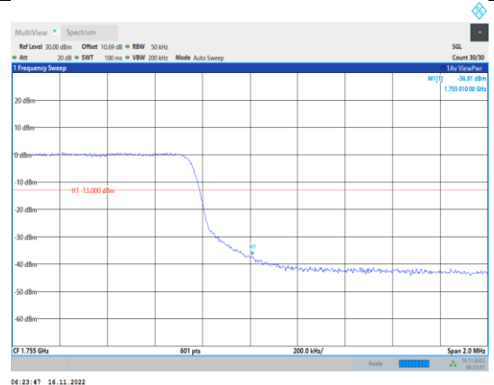
Band4-5MHz-64QAM-20375-25RB#0
