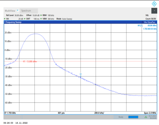
Band4-10MHz-64QAM-20350-1RB#49
