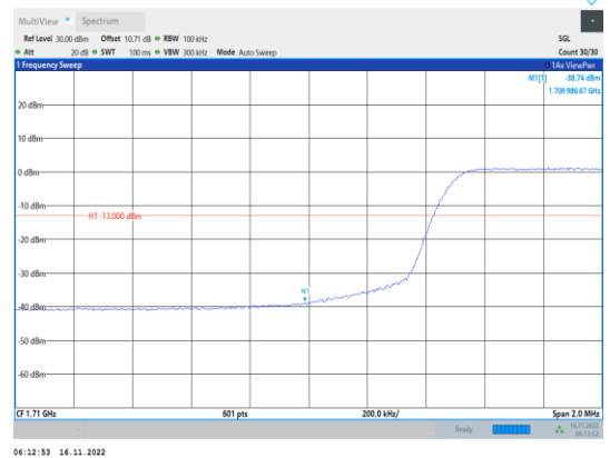
Band4-10MHz-64QAM-20000-50RB#0
