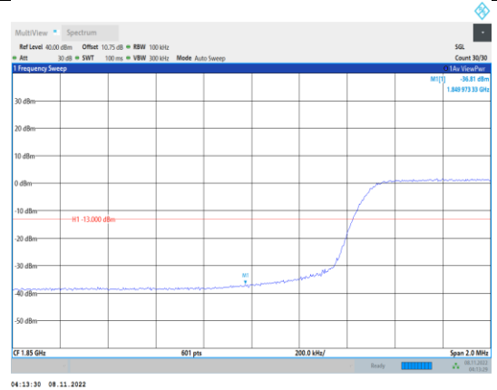
Band2-10MHz-16QAM-18650-50RB#0
