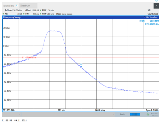
Band4-5MHz-16QAM-20375-1RB#24
