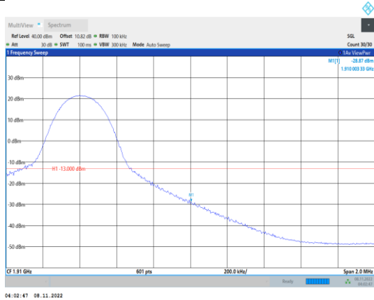
Band2-10MHz-QPSK-19150-1RB#49
