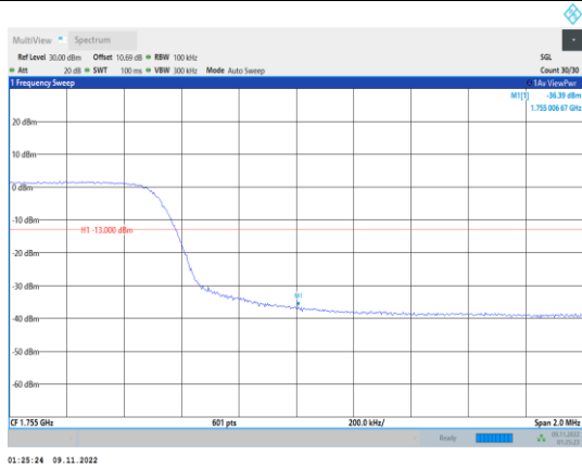
Band4-10MHz-16QAM-20350-50RB#0
