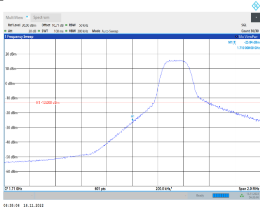
Band4-5MHz-64QAM-19975-1RB#0
