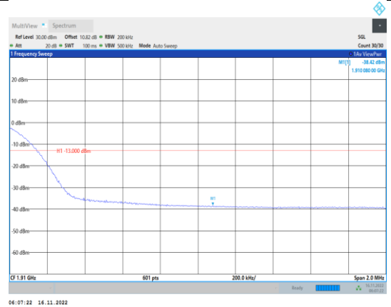
Band2-20MHz-64QAM-19100-100RB#0
