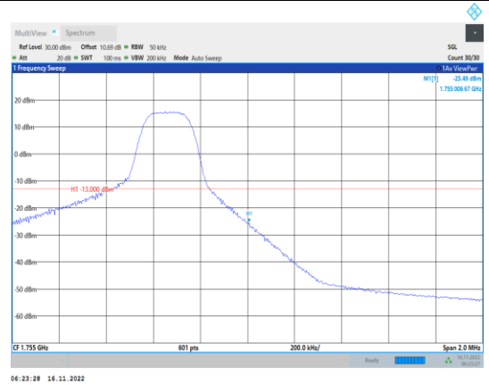
Band4-5MHz-64QAM-20375-1RB#24
