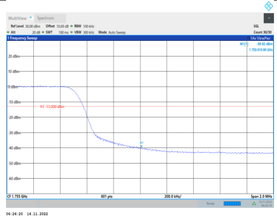
Band4-10MHz-64QAM-20350-50RB#0
