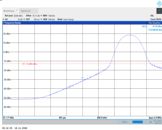
Band4-10MHz-64QAM-20000-1RB#0
