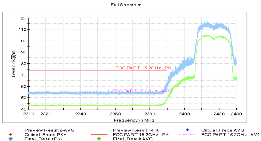
Fig.A.6.2.12 Transmitter Spurious Emission - Radiated (Power): 802.11ax-HT20, ch2, 2.31 GHz - 2.43GHz
