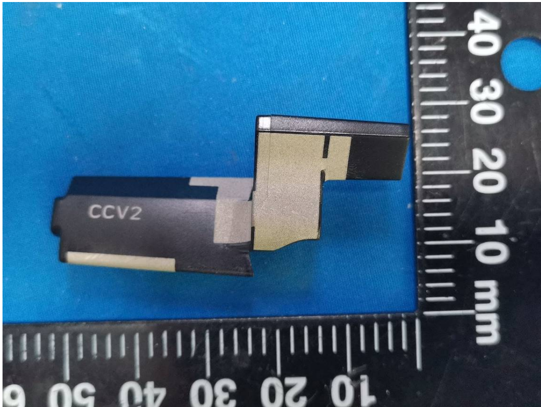
3G/4G Main Antenna
