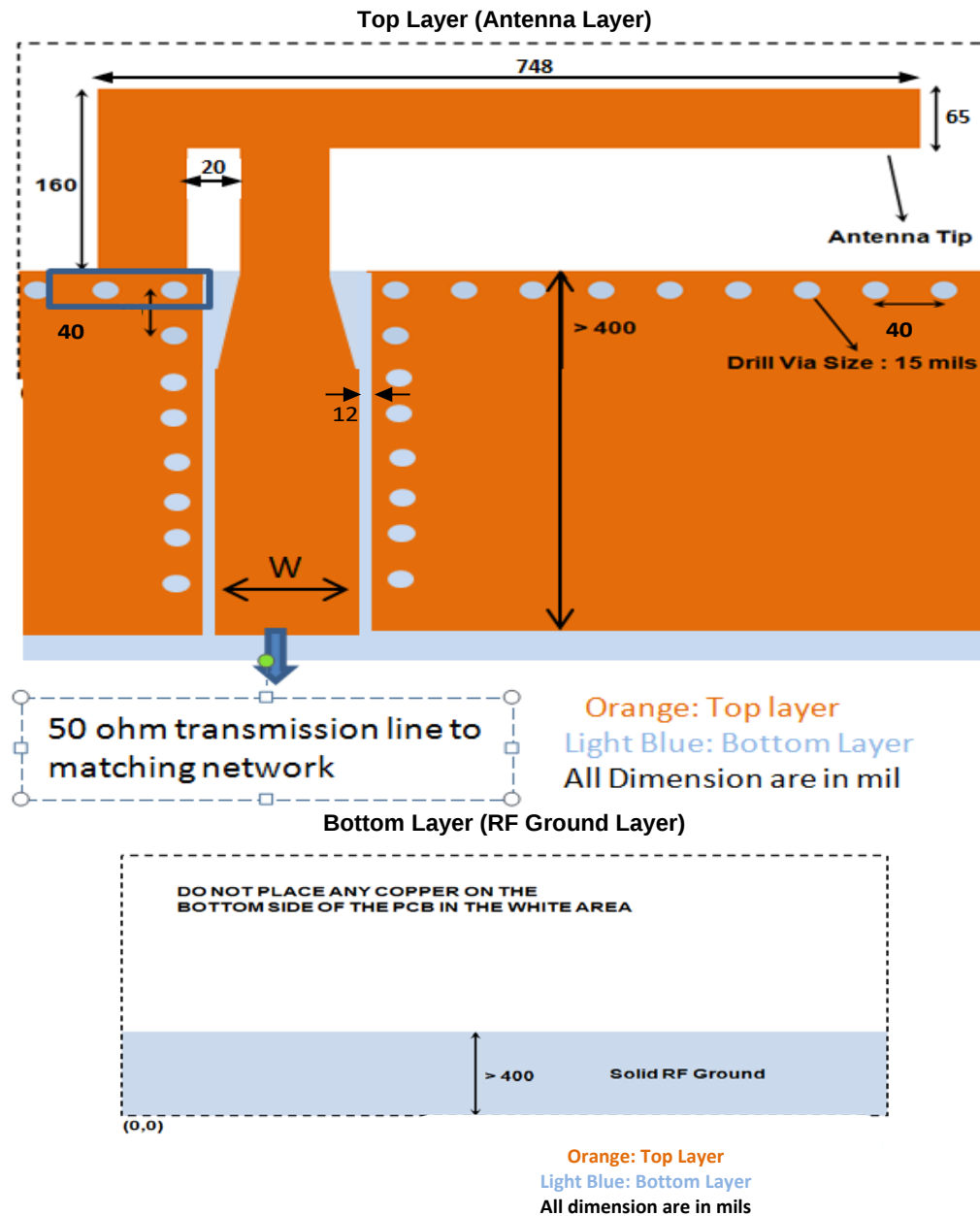
Figure 16. IFA Layout
