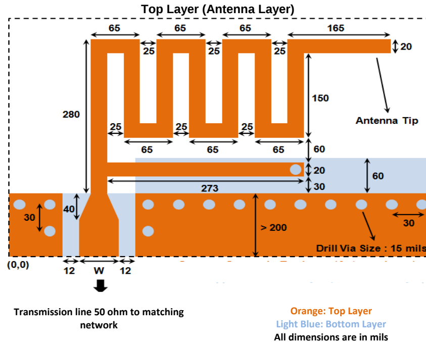
Figure 10. MIFA Layout
