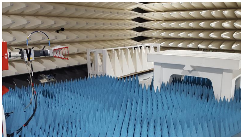
Figure B4. High range Radiated emission Set up Horn antenna
