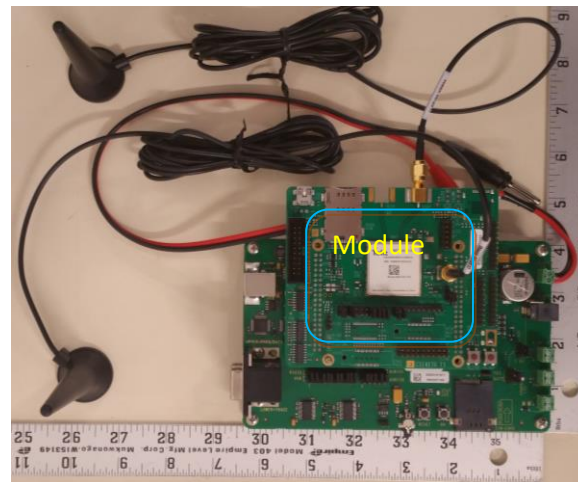
Figure B1. DUT with its accessories and Evaluation Kit top view
