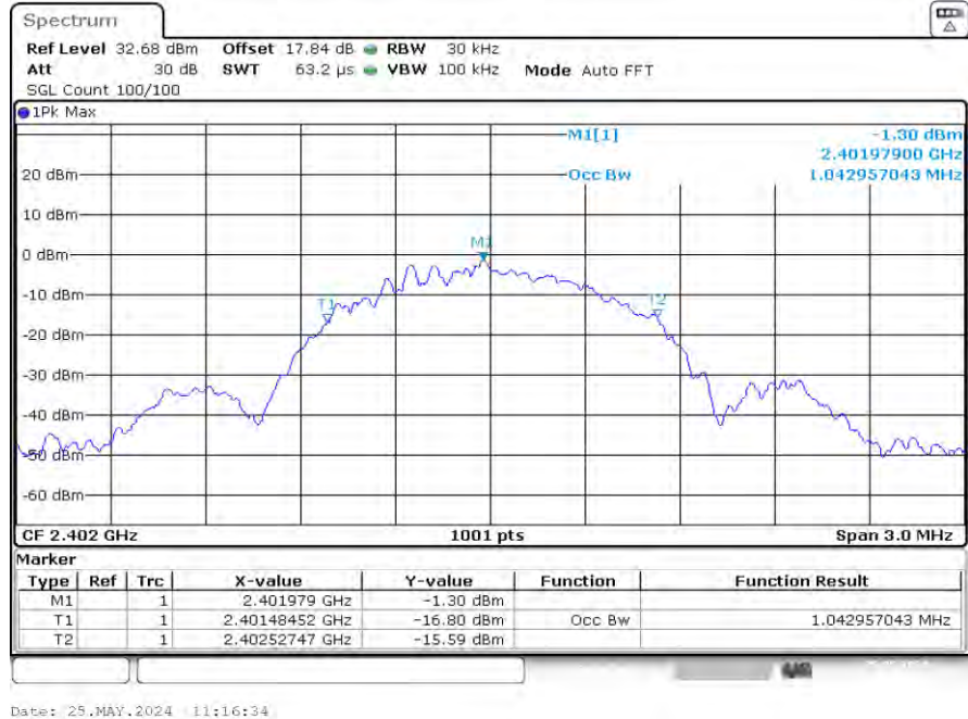
99%_Occupied_Bandwidth_NVNT_ANT1_1Mbps_2402
