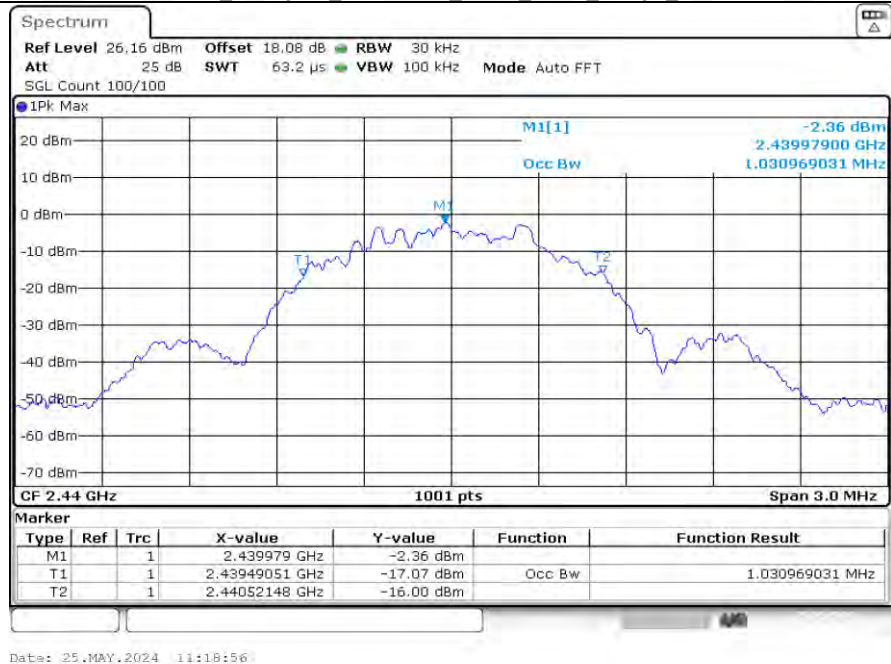
99%_Occupied_Bandwidth_NVNT_ANT1_1Mbps_2440
