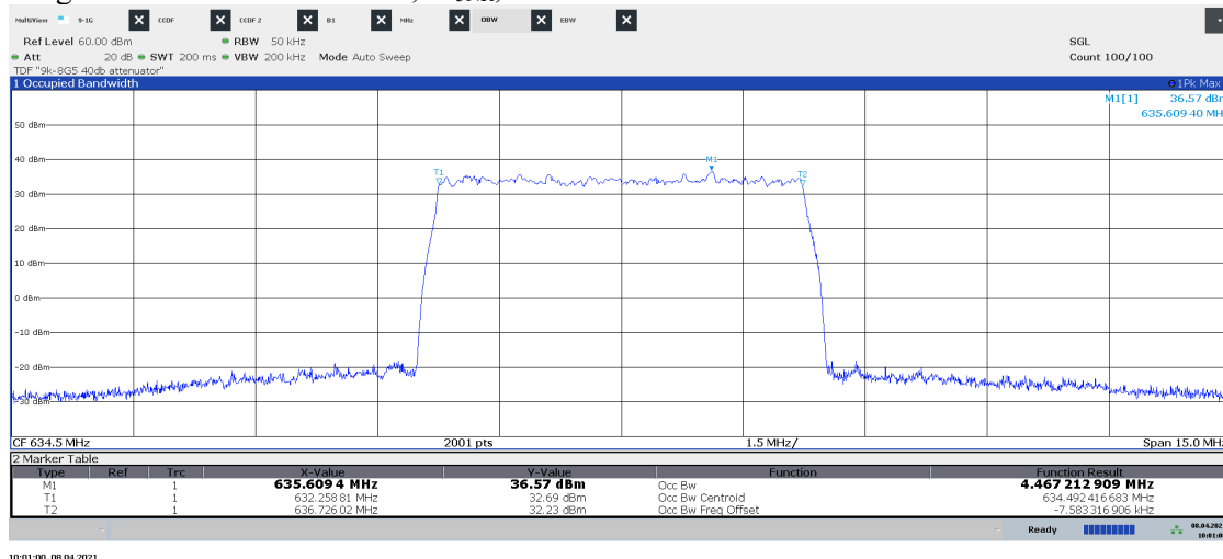
Diagram 1.12 NR: RF1-TM3.1, M 5NR , Port B:
