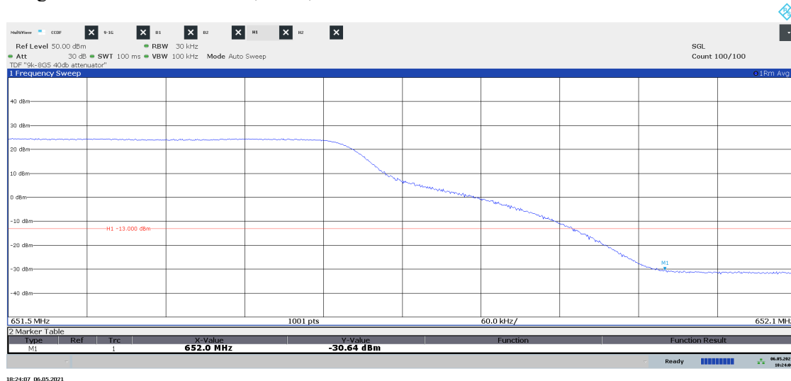
Diagram 2.20a LTE: ETM1.1, T SLTE , Port C:
