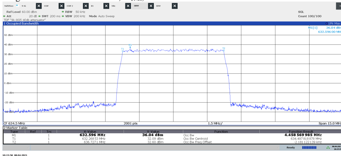
Diagram 1.13 NR: RF1-TM3.1a, M 5NR , Port B:
