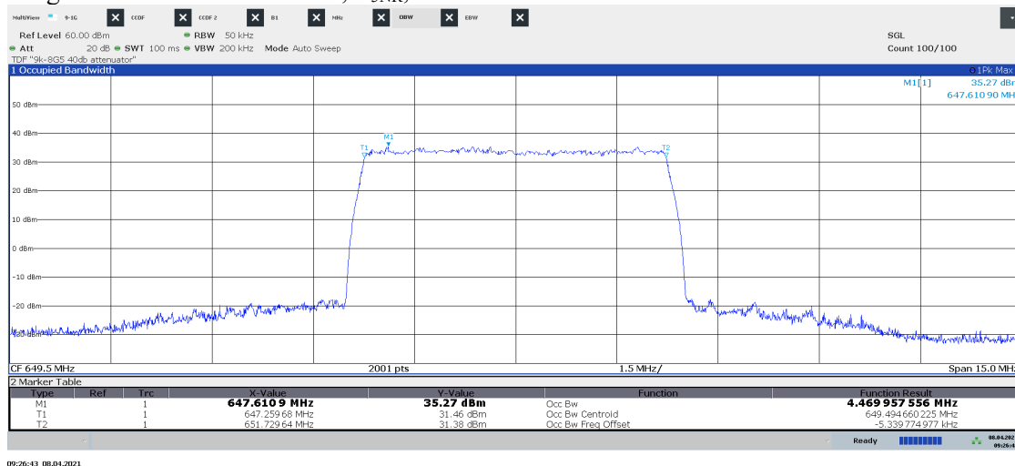
Diagram 1.10 NR: RF1-TM1.1, T 5NR , Port B:
