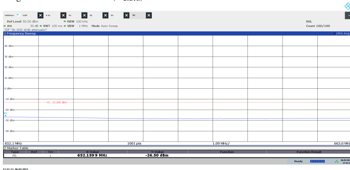
Diagram 2.24b LTE: ETM1.1, T_{20\text{LTE}} , Port B:
