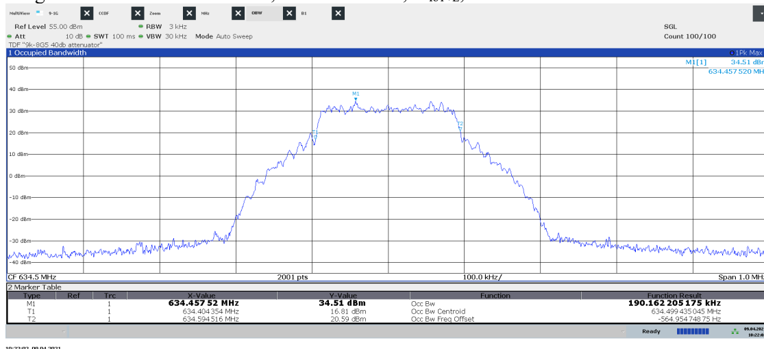
Diagram 1.24 NB IoT SA N-TM, LTE: E-TM1.1, M_{IoT+L} , Port A:
