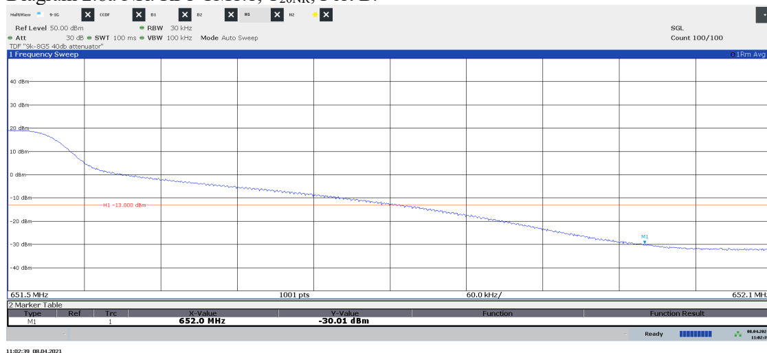
Diagram 2.8a NR: RF1-TM1.1, T 20NR , Port B:
