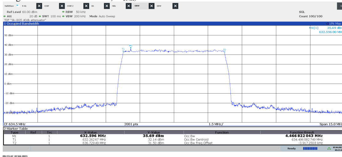
Diagram 1.4 NR: RF1-TM1.1, M 5NR , Port B:
