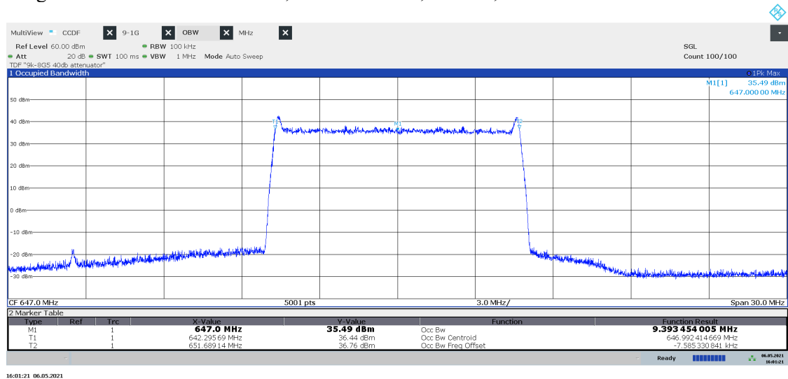
Diagram 1.28 NB IoT GB: N-TM, LTE: E-TM3.1, T10_{Guard} , Port B:
