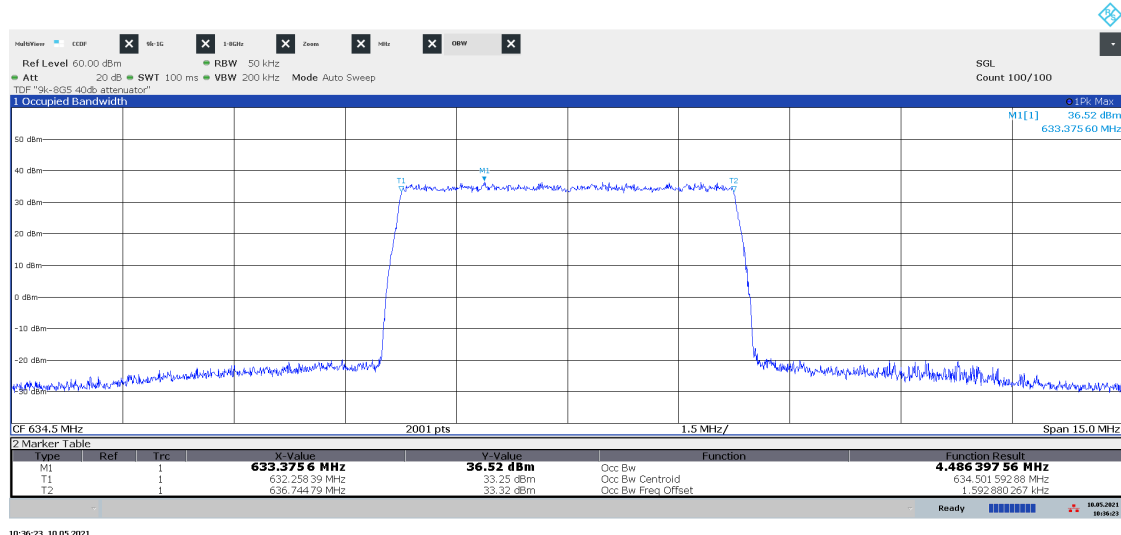
Diagram 1.21 LTE: ETM3.1a, M 5LTE , Port B:
