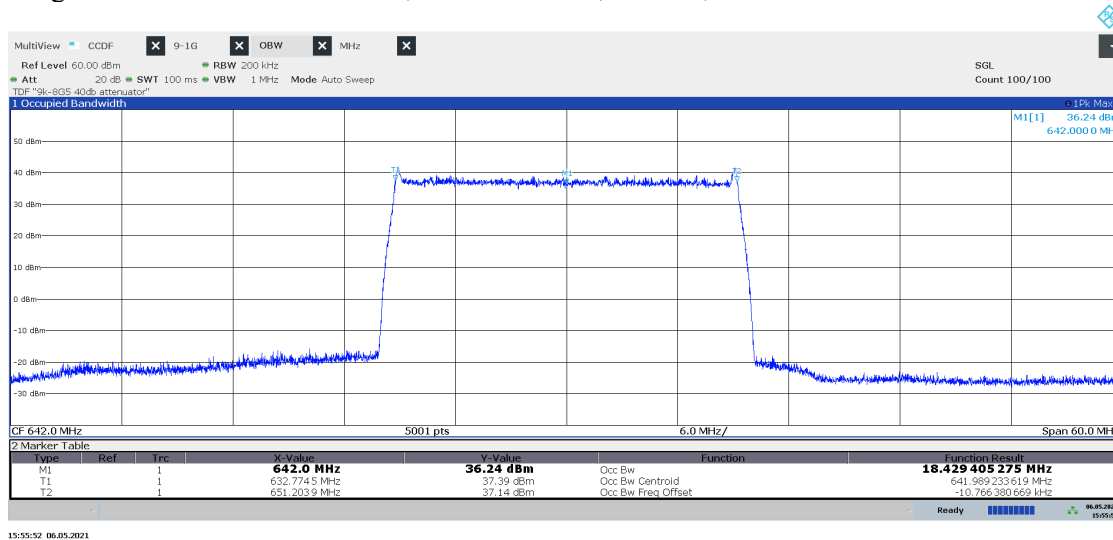
Diagram 1.30 NB IoT GB: N-TM, LTE: E-TM3.1, T20 Guard , Port B:
