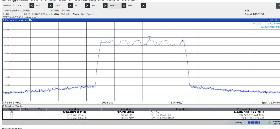
Diagram 1.14 NR: RF1-TM3.2, M 5NR , Port B:
