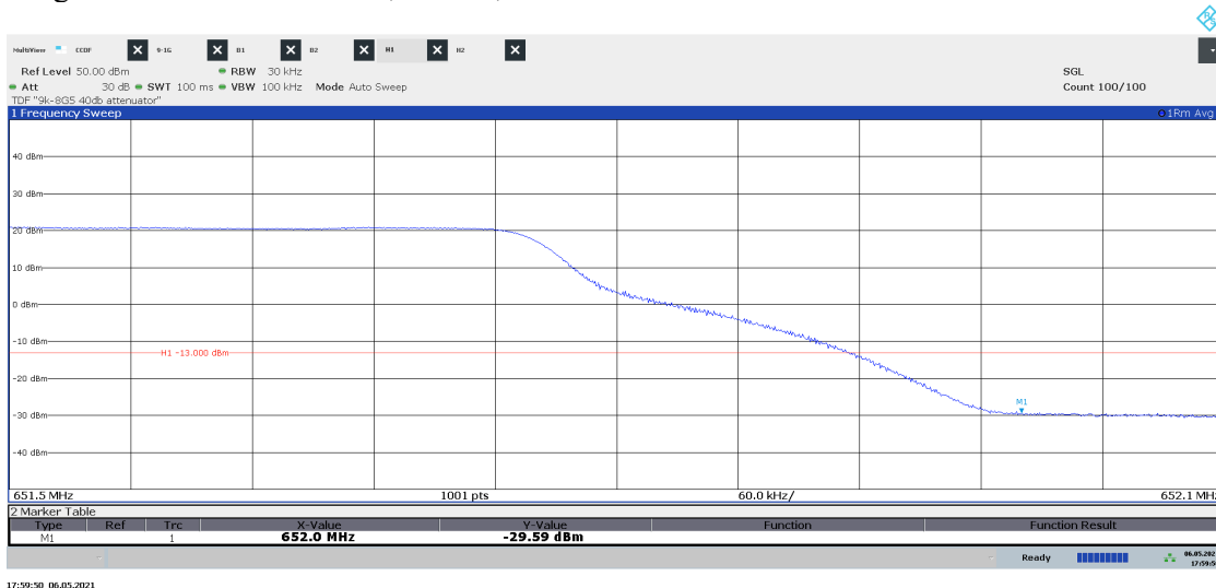
Diagram 2.26a LTE: ETM1.1, Tim LTE , Port B:
