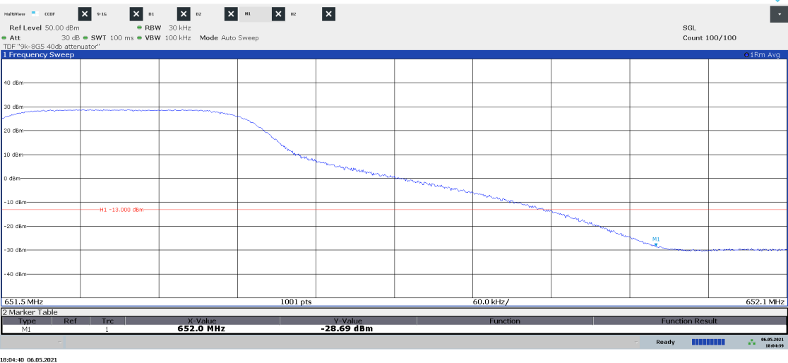
Diagram 2.34a NB IoT SA: N-TM, LTE: E-TM3.1, T10 Guard , Port B:
