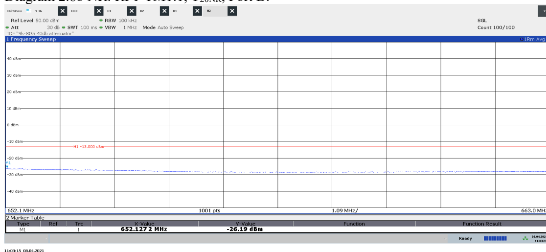
Diagram 2.8b NR: RF1-TM1.1, T 20NR , Port B:
