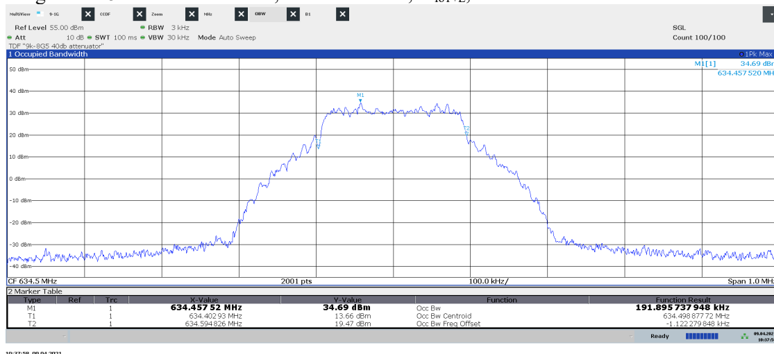
Diagram 1.25 NB IoT SA N-TM, LTE: E-TM1.1, M_{IoT+L} , Port B:
