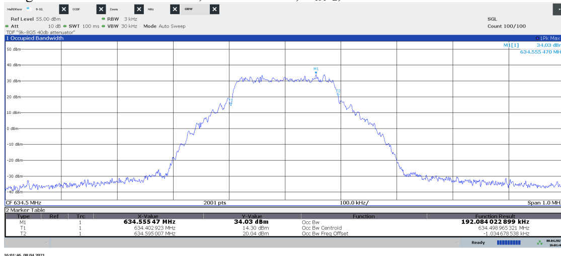
Diagram 1.26 NB IoT SA N-TM, LTE: E-TM1.1, M_{IoT+L} , Port C:
