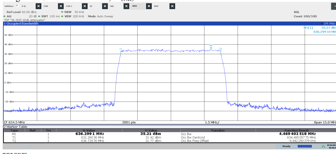
Diagram 1.5 NR: RF1-TM1.1, M 5NR , Port C:
