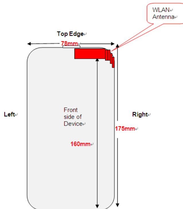
Distance of EUT antenna-to-edge/surface(mm), Test distance:10mm
