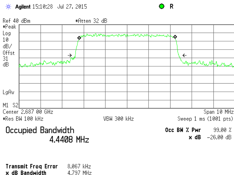
Plot 7.1.6 Occupied bandwidth test results at high frequency, 5 MHz EBW, 64QAM, RF#2
