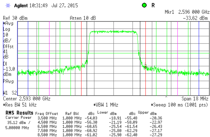
Plot 7.3.6 Spurious emission at band edges test results at high carrier frequency, 5 MHz EBW
