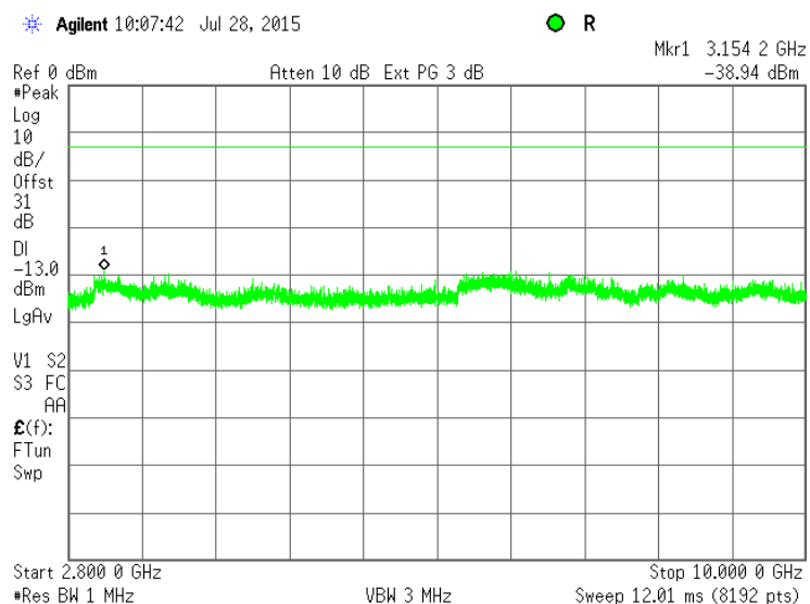
Plot 7.4.19 Spurious emission measurements in 2800 - 10000 MHz range at low carrier frequency, #RF2
