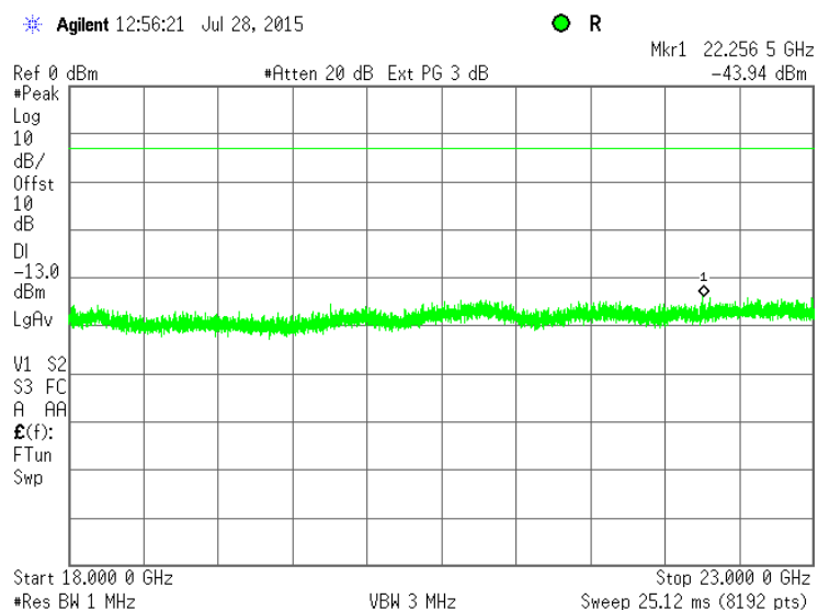
Plot 7.4.25 Spurious emission measurements in 18000 - 23000 MHz at low carrier frequency, #RF2
