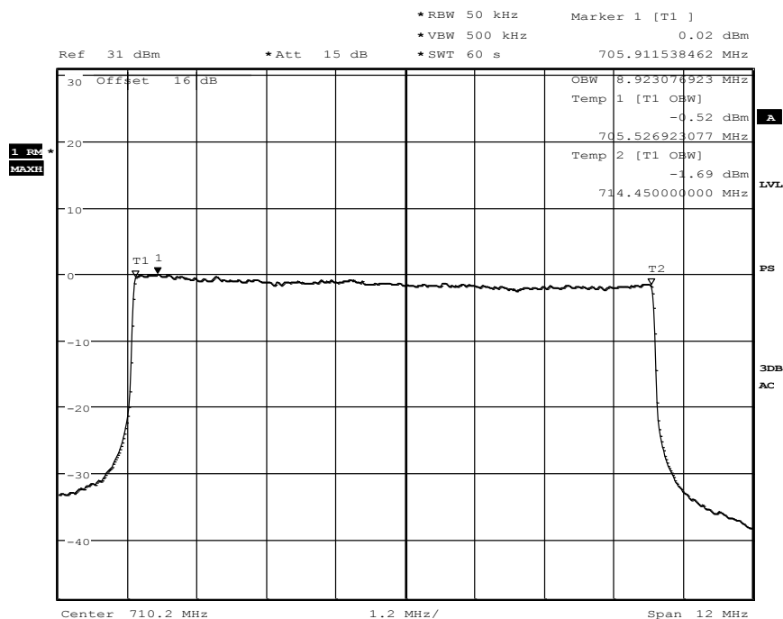
Diagram 35.171, QPSK-Modulation
