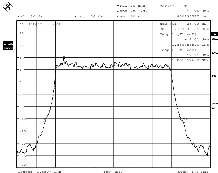
Diagram 34.200, QPSK-Modulation
