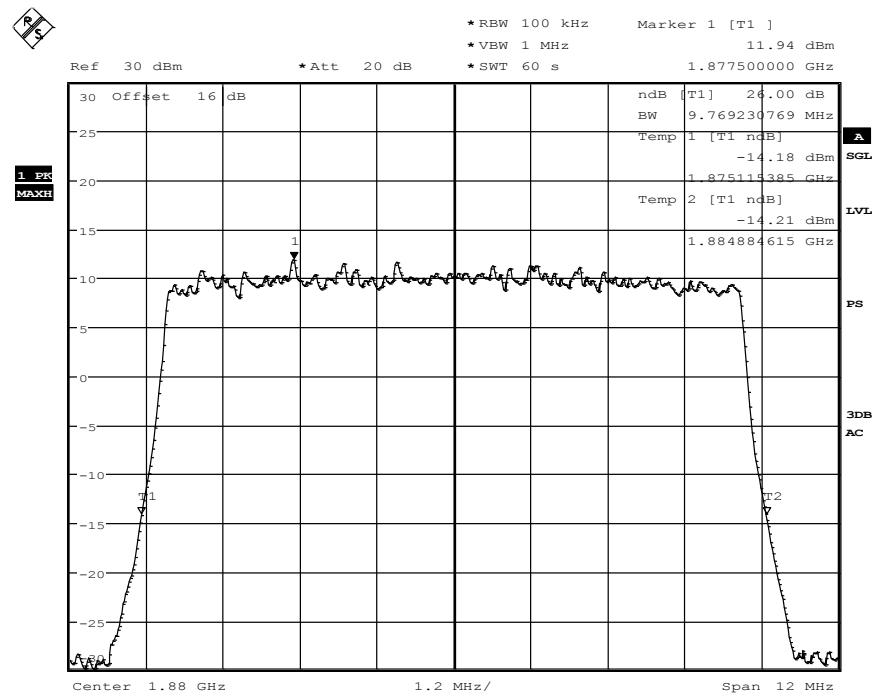
Diagram 34.209, QPSK-Modulation
