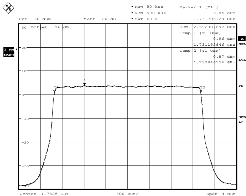
Diagram 35.404, QPSK-Modulation
