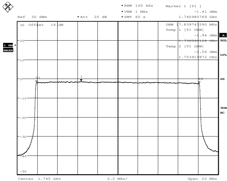
Diagram 35.418, QPSK-Modulation
