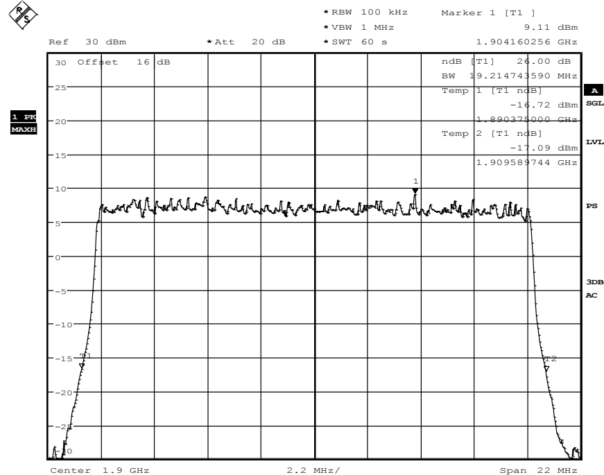
Diagram 34.217, QPSK-Modulation
