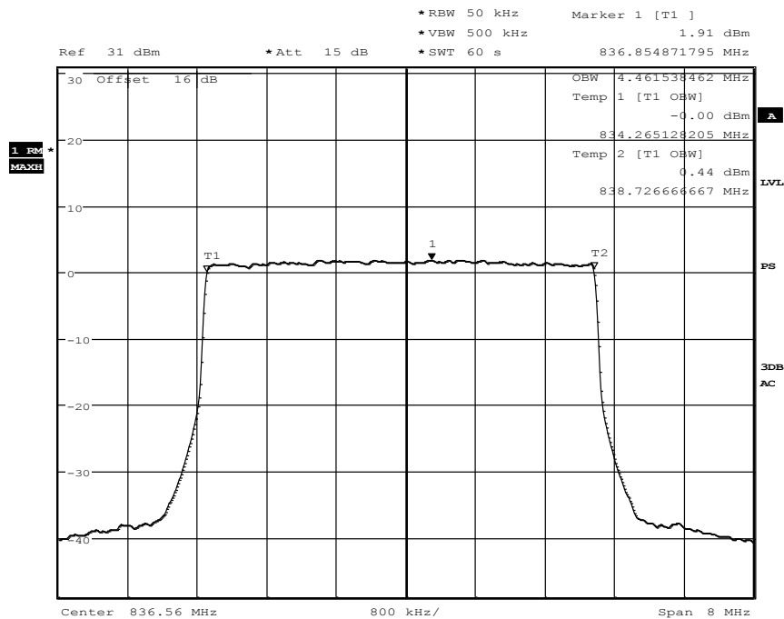
Diagram 35.509, QPSK-Modulation
