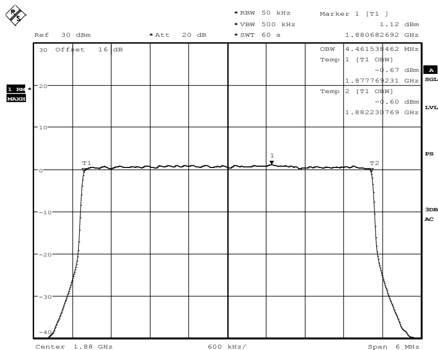
Diagram 35. 207, QPSK-Modulation
