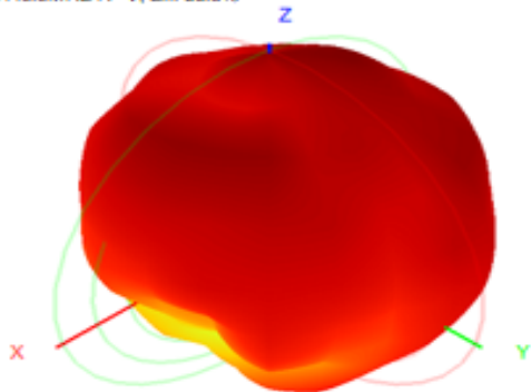
2440.0MHz H+V, Eff: 53.6%
