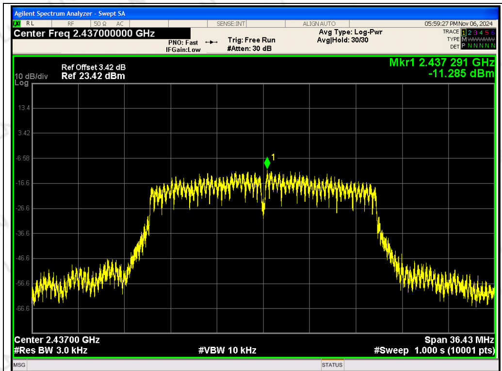
ANT 2 TX 802.11n/HT20 CH06: 2437MHz
