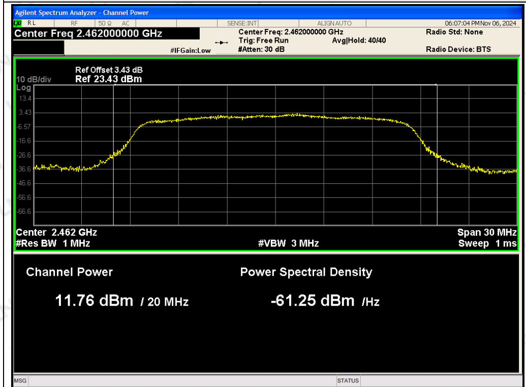
ANT 2 802.11g 2462MHz
