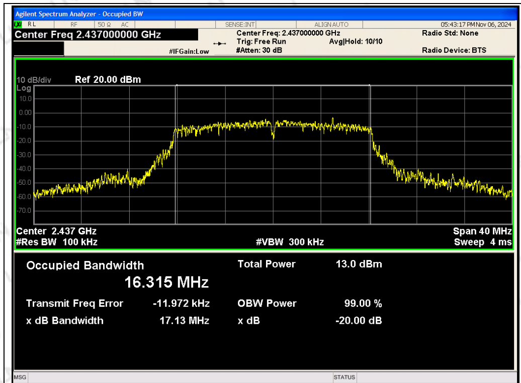
ANT 1 TX 802.11g CH06: 2437MHz
