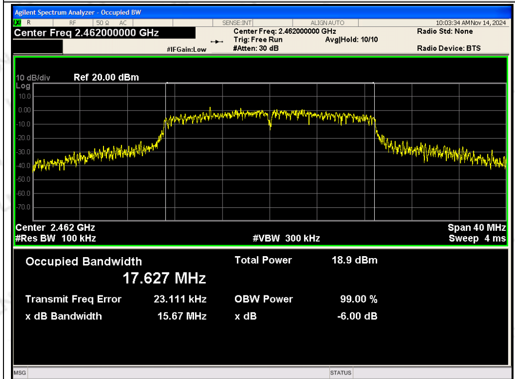
ANT 1 TX 802.11n/HT20 CH11: 2462MHz
