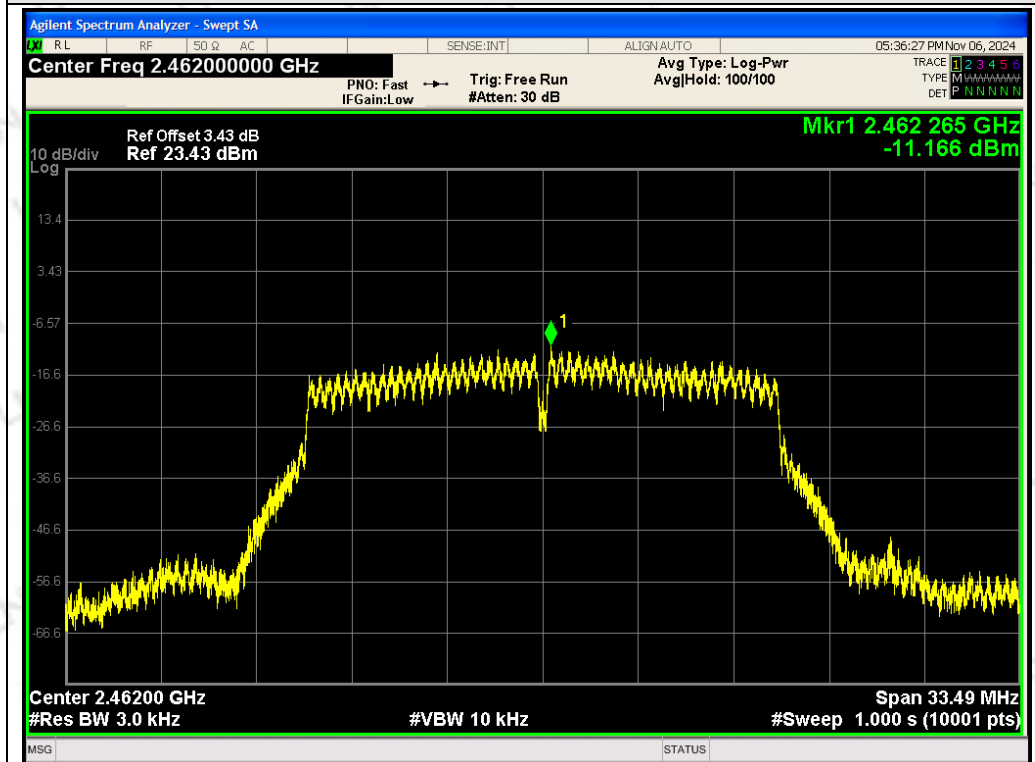
ANT 1 TX 802.11g CH11: 2462MHz
