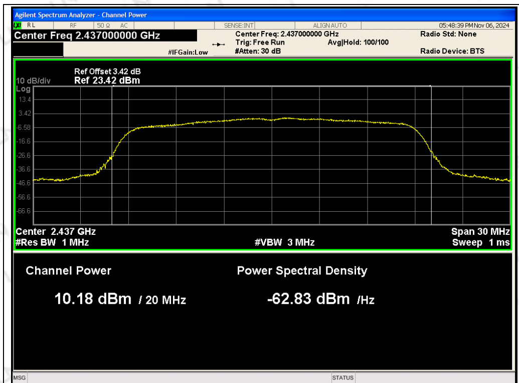
ANT 1 802.11n/HT20 2437MHz
