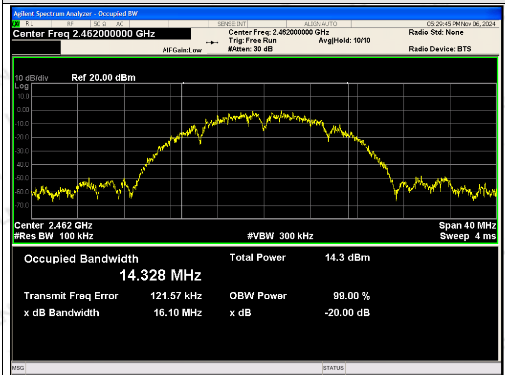
ANT 1 TX 802.11b CH11: 2462MHz
