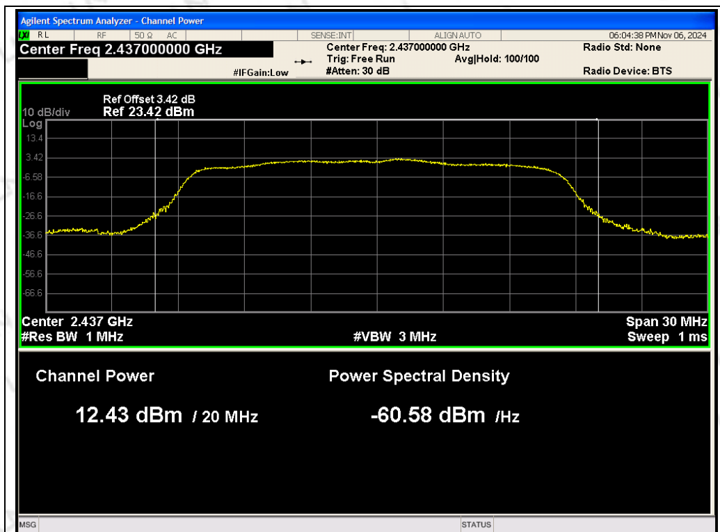
ANT 2 802.11g 2437MHz
