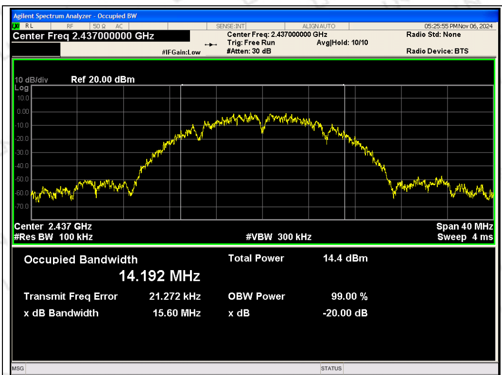
ANT 1 TX 802.11b CH06: 2437MHz
