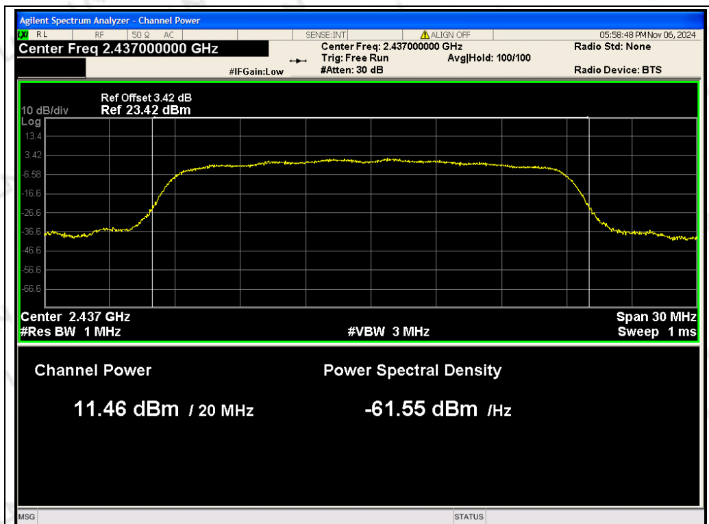
ANT 2 802.11n/HT20 2437MHz
