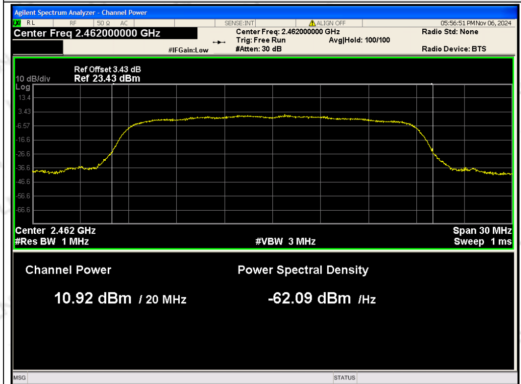
ANT 2 802.11n/HT20 2462MHz
