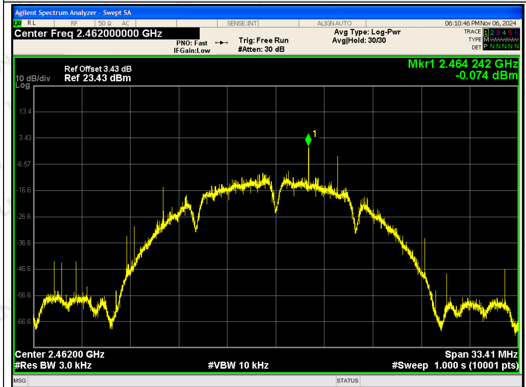
ANT 2 TX 802.11b CH11: 2462MHz
