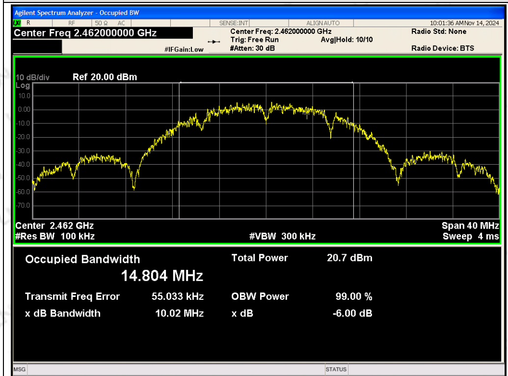
ANT 1 TX 802.11b CH11: 2462MHz
