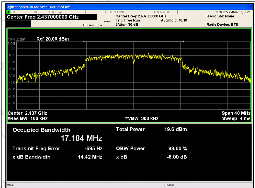
ANT 2 TX 802.11g CH06: 2437MHz
