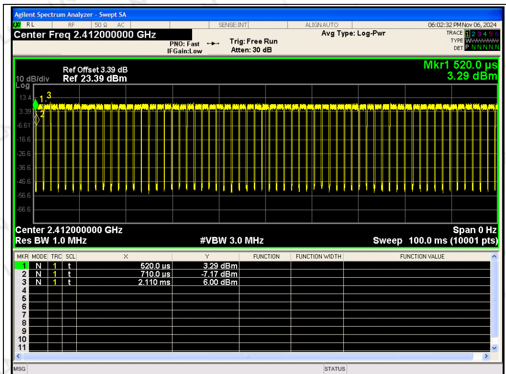
ANT 2 802.11g 2412MHz
