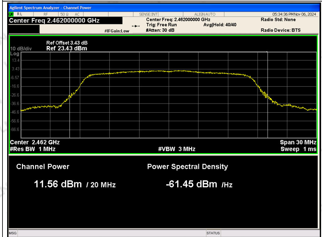
ANT 1 802.11g 2462MHz
