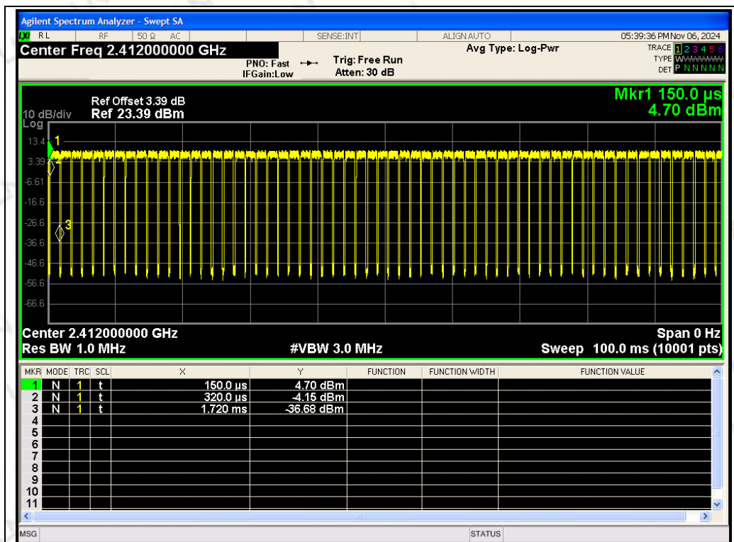
ANT 1 802.11g 2412MHz
