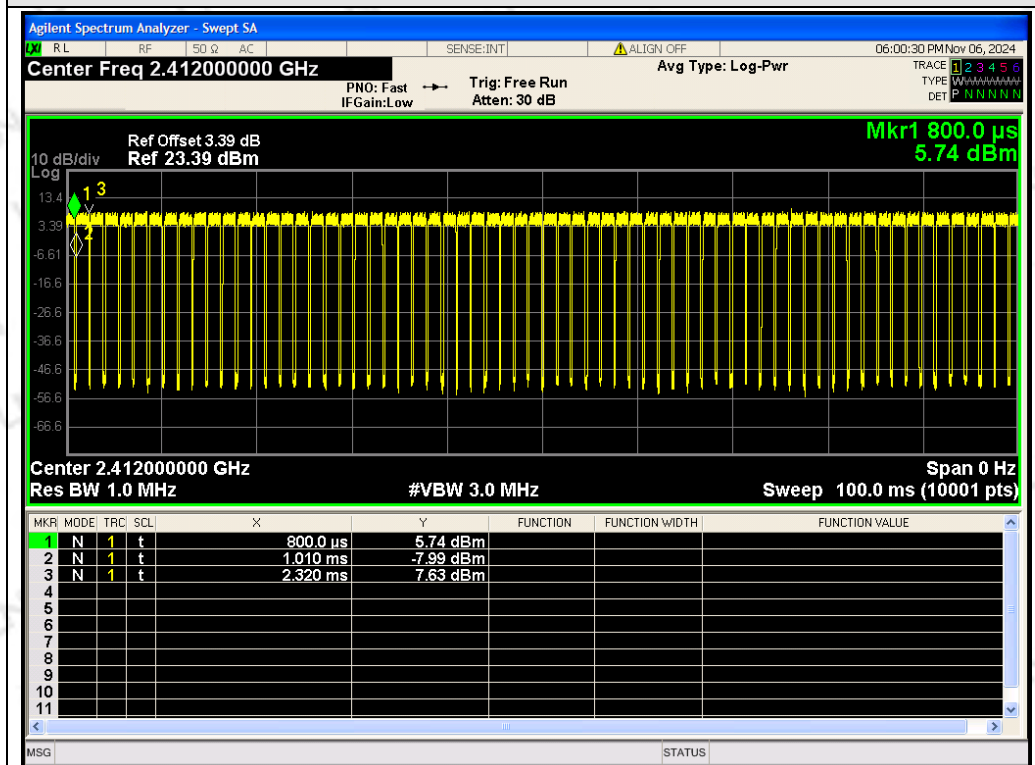
ANT 2 802.11n/HT20 2412MHz
