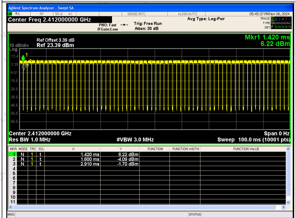
ANT 1 802.11n/HT20 2412MHz
