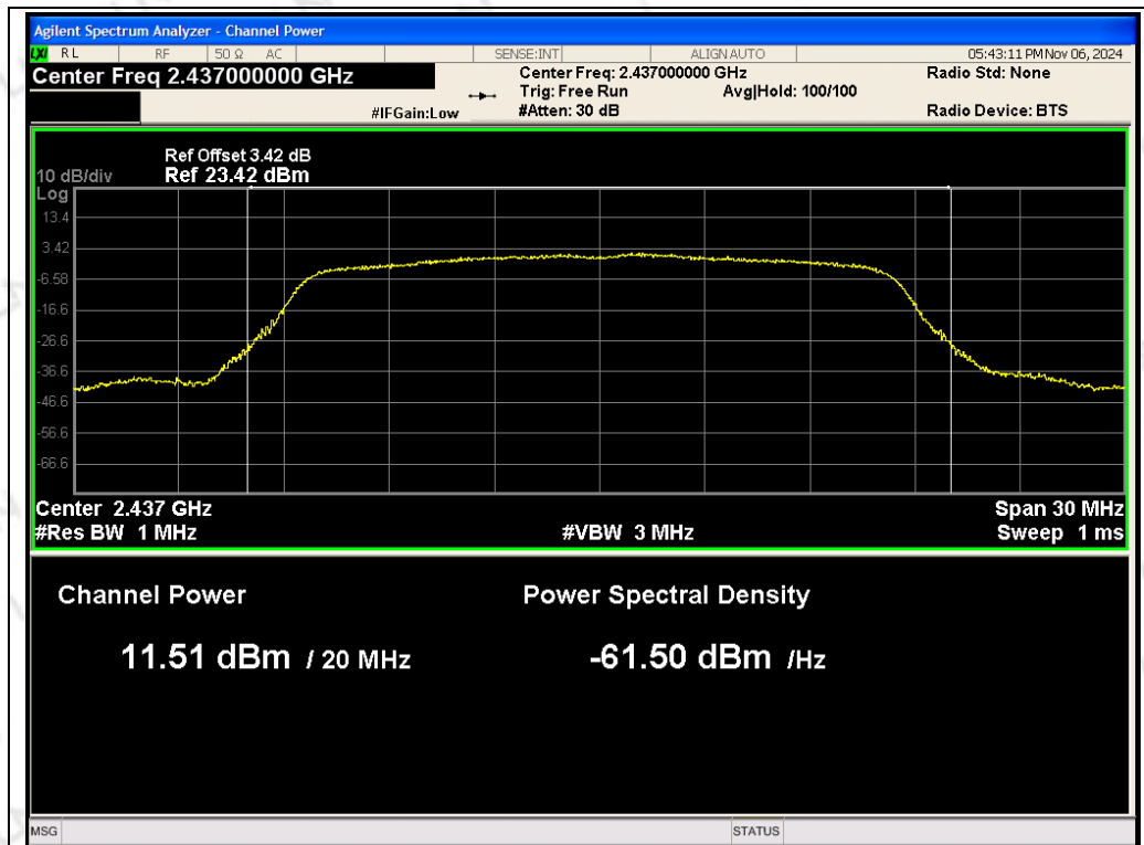
ANT 1 802.11g 2437MHz
