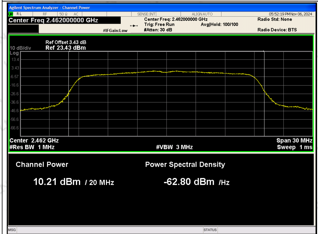
ANT 1 802.11n/HT20 2462MHz
