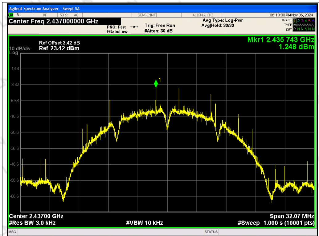
ANT 2 TX 802.11b CH06: 2437MHz
