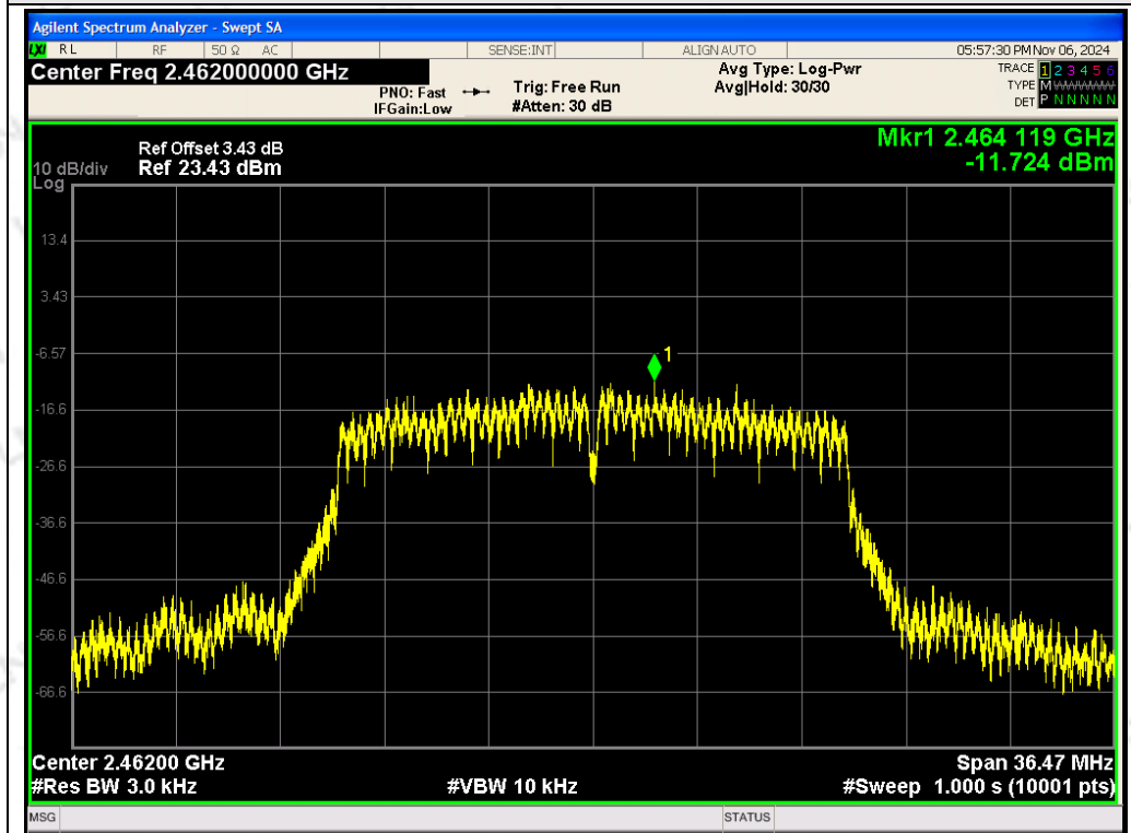
ANT 2 TX 802.11n/HT20 CH11: 2462MHz
