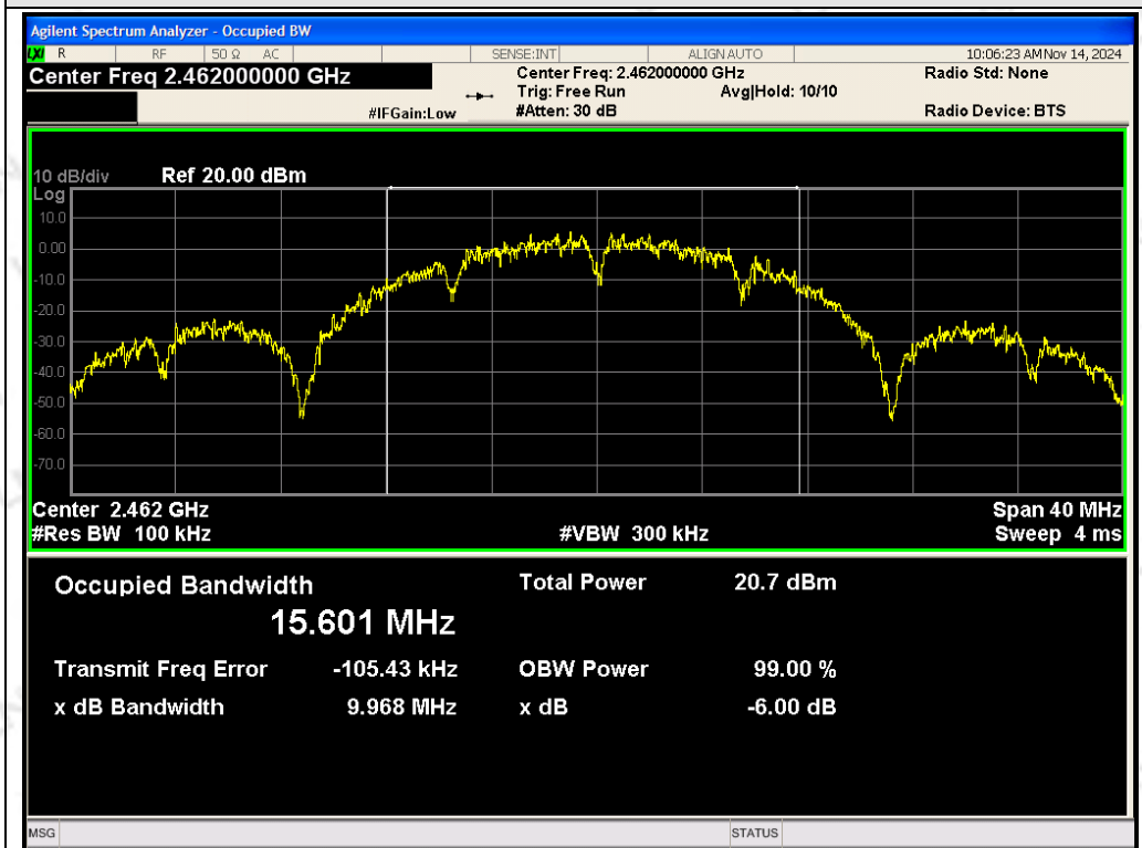
ANT 2 TX 802.11b CH11: 2462MHz
