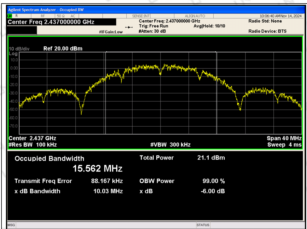
ANT 2 TX 802.11b CH06: 2437MHz
