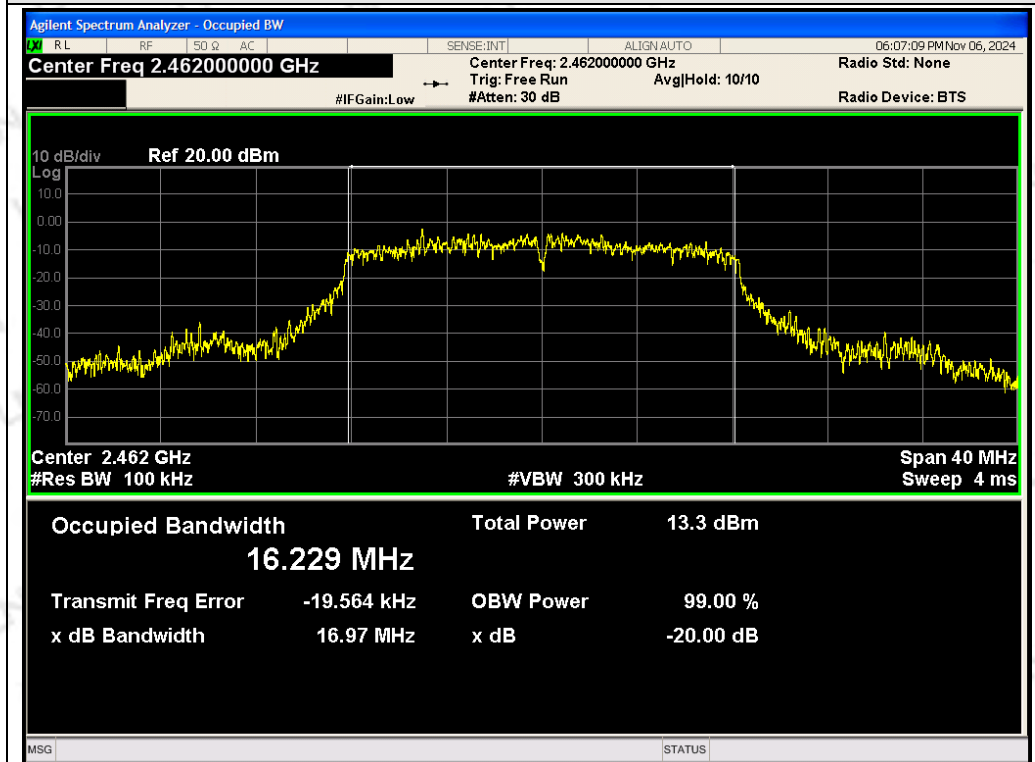
ANT 2 TX 802.11g CH11: 2462MHz
