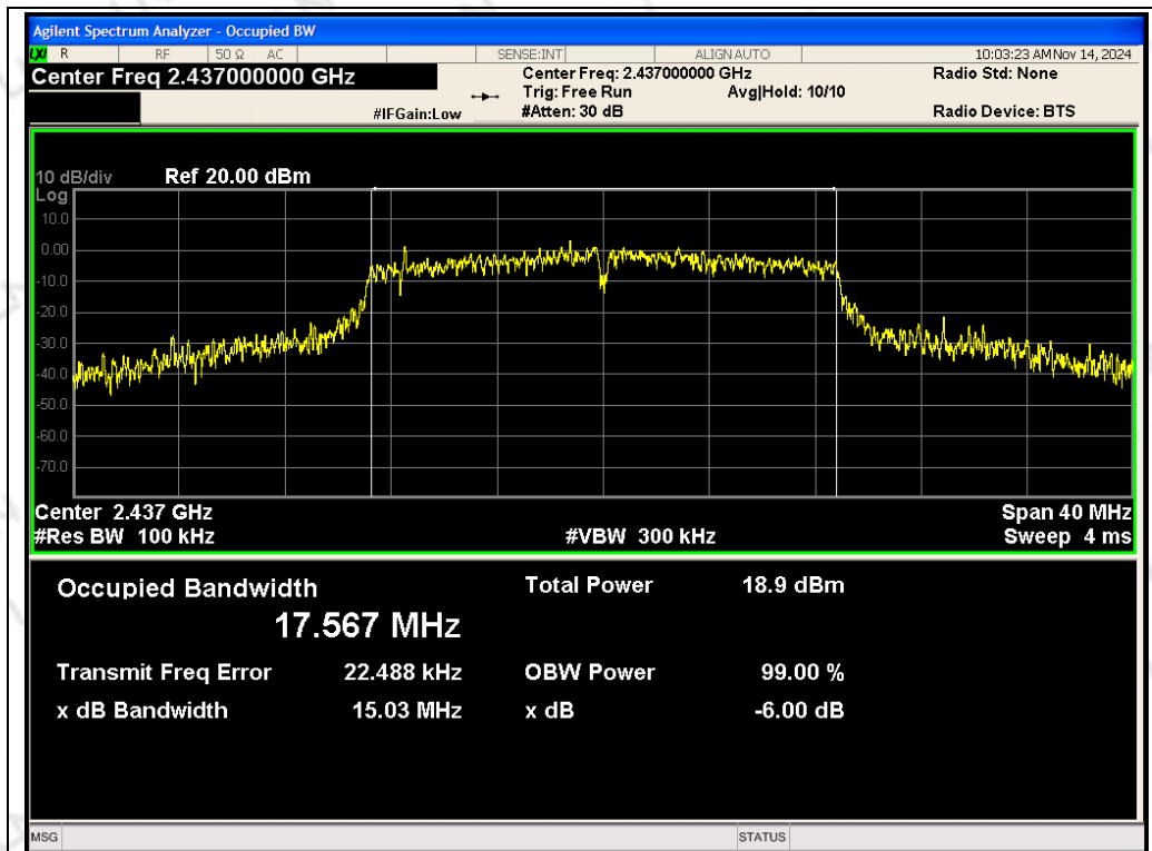
ANT 1 TX 802.11n/HT20 CH06: 2437MHz
