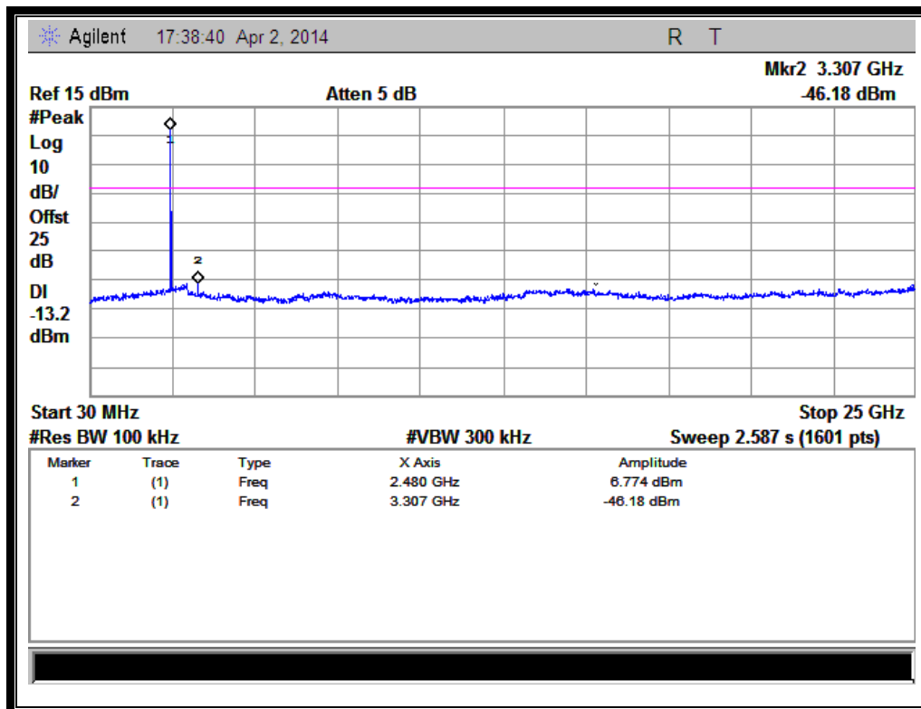
(Plot F.1: Channel = 78, 30MHz to 25GHz @ 1/4-DQPSK)
