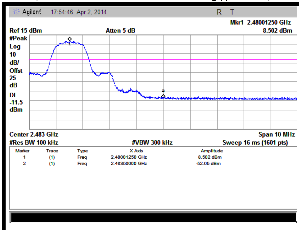
(Channel = 78, Band edge @ 1/4-DQPSK)
