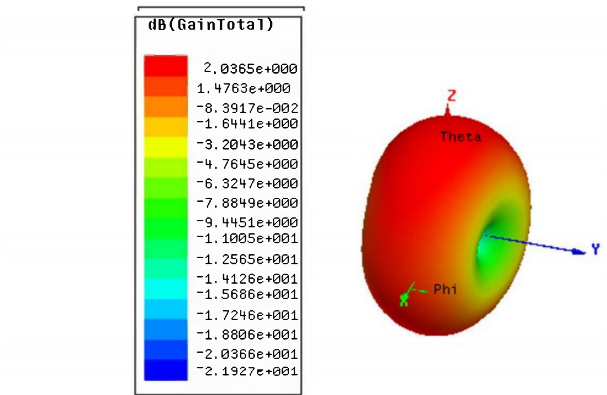
Radiation Figure
