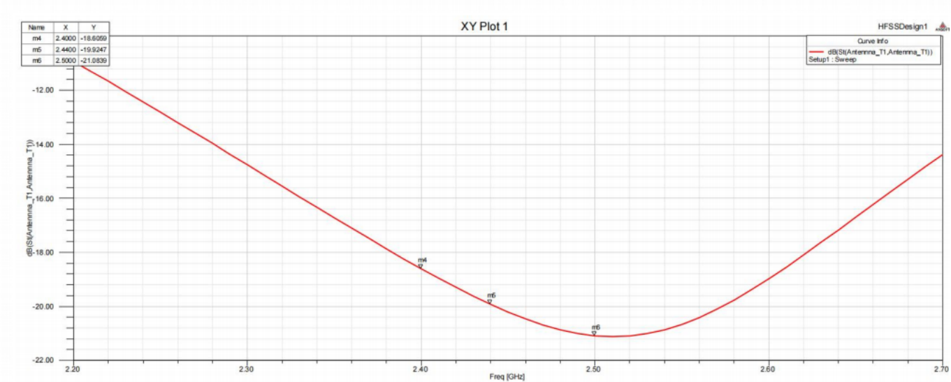
S11 Figure
