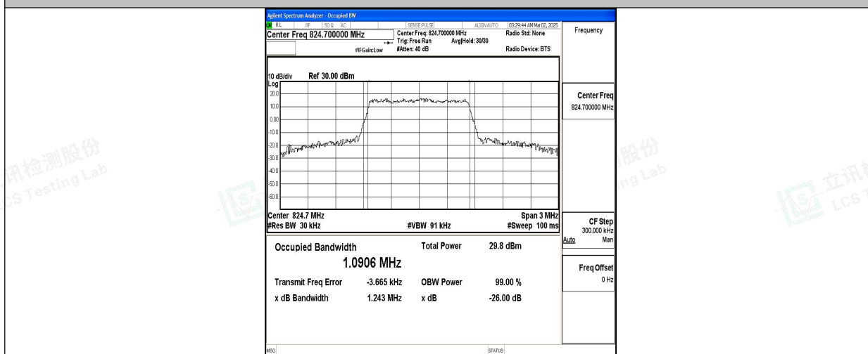
Band5-1.4MHz-16QAM-20407-6RB#0-PASS
