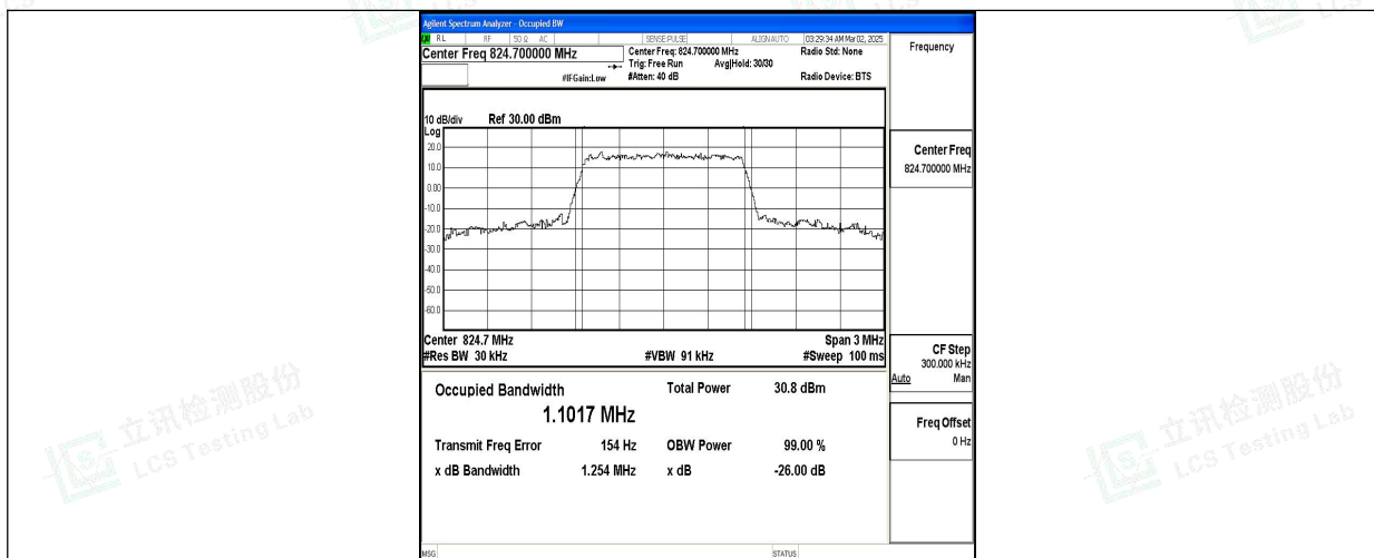
Band5-1.4MHz-QPSK-20407-6RB#0-PASS
