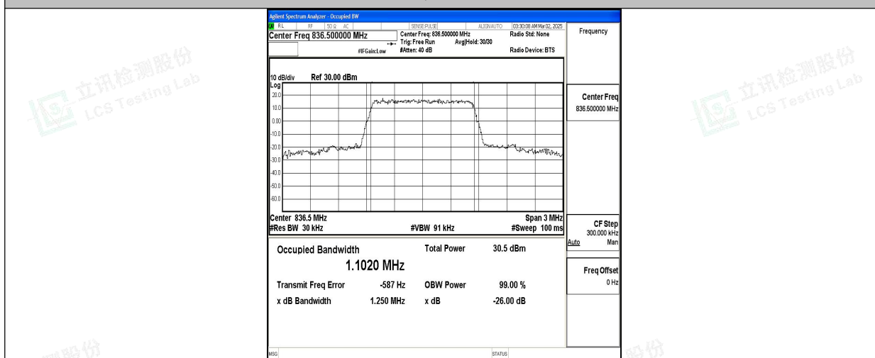
Band5-1.4MHz-QPSK-20525-6RB#0-PASS
