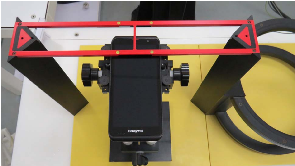
Picture 1: Test Setup
