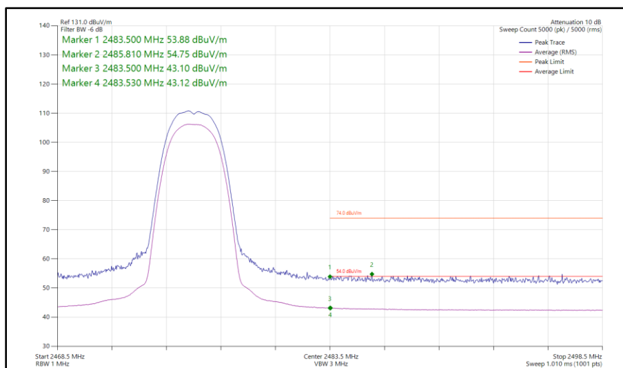
Figure 65 - Bluetooth HDR4, MIMO, Core 0 - Core 1 - 2476 MHz Band Edge Frequency 2483.5 MHz
