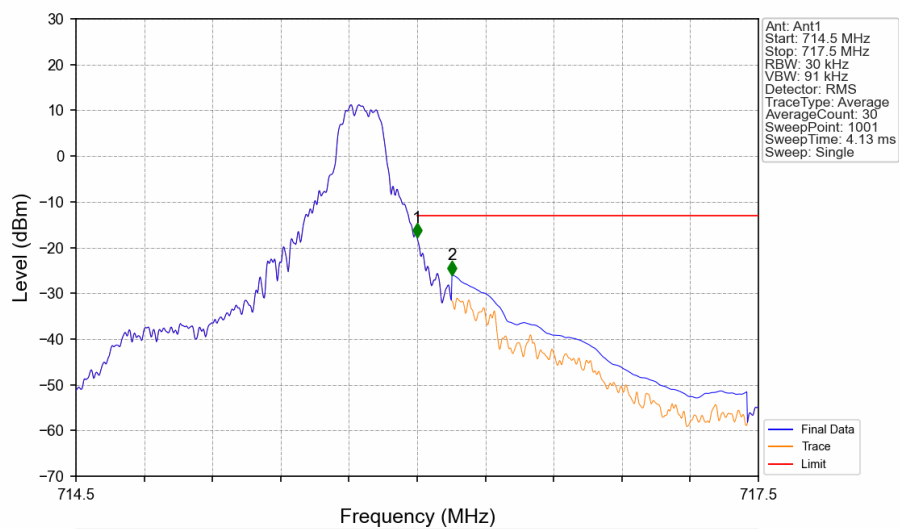
Band12_1.4MHz_QPSK_HCH_715.3MHz_RB_1_5_NTNV
