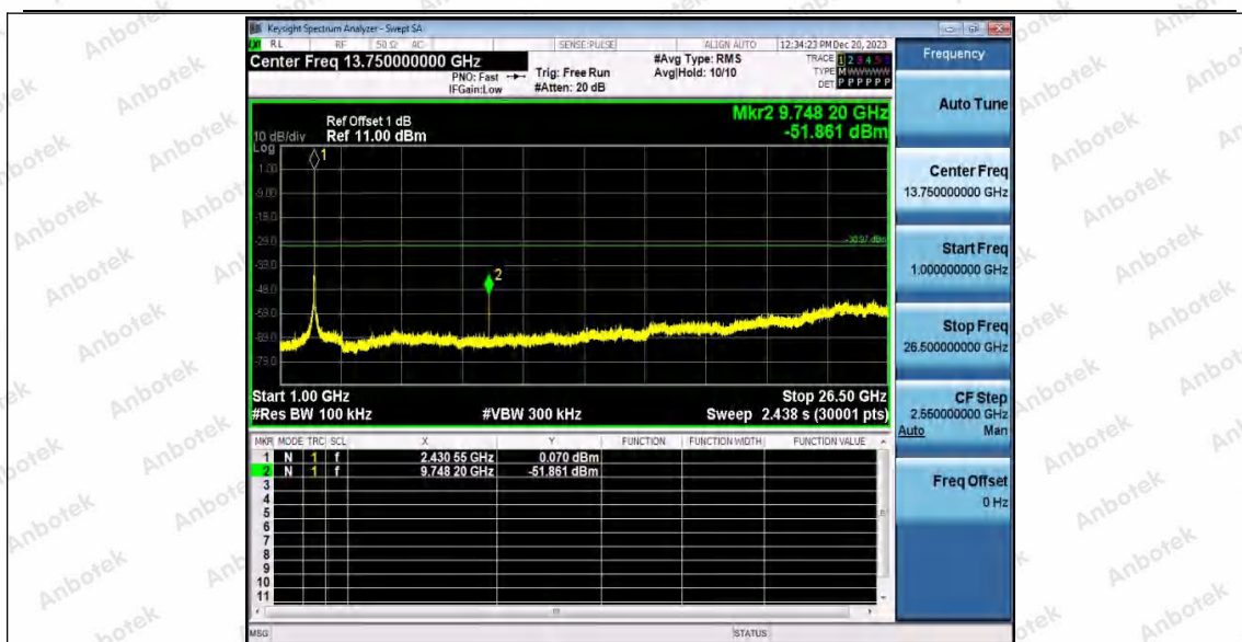
11G_WiFi 1_2437_0~Reference
