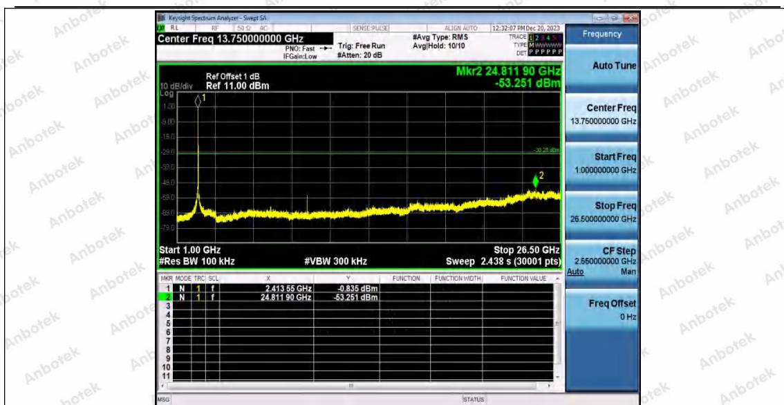
11G_WiFi 1_2412_0~Reference
