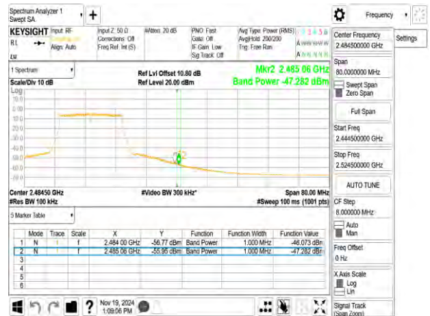
802.11g_20MHz_2467MHz
