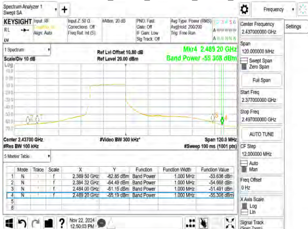
802.11ax_40MHz_2437MHz_RU242_62
