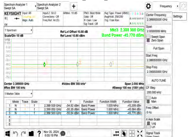
802.11ax_40MHz_2432MHz_RU242_61
