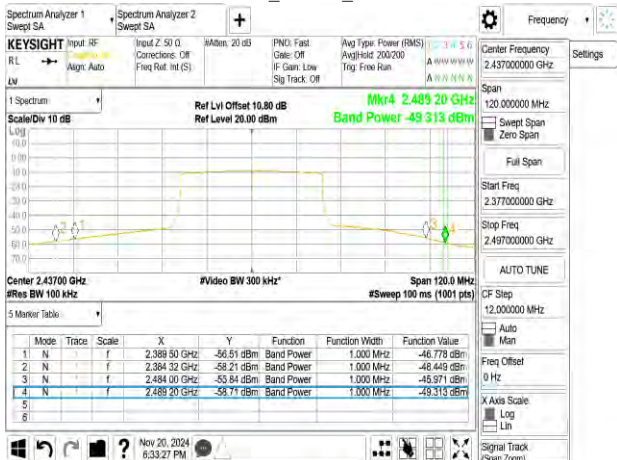
802.11ax_40MHz_2437MHz_RU242_61
