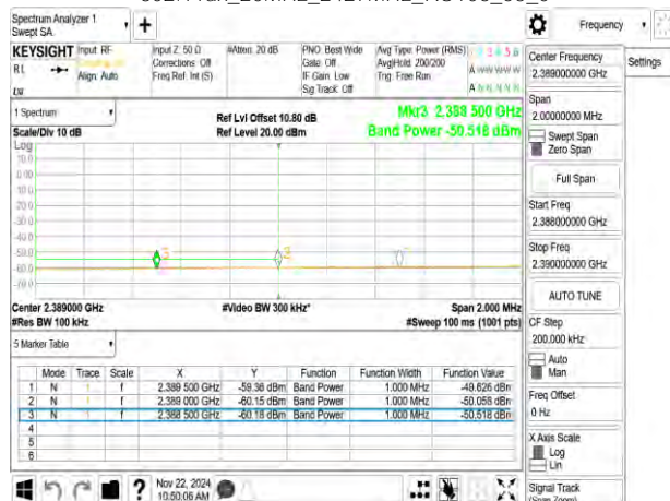
802.11ax_20MHz_2427MHz_RU106_53_0
