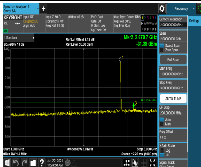
Band7-10MHz-16QAM-20800-1RB#0-Range5:3000~26500MHz
