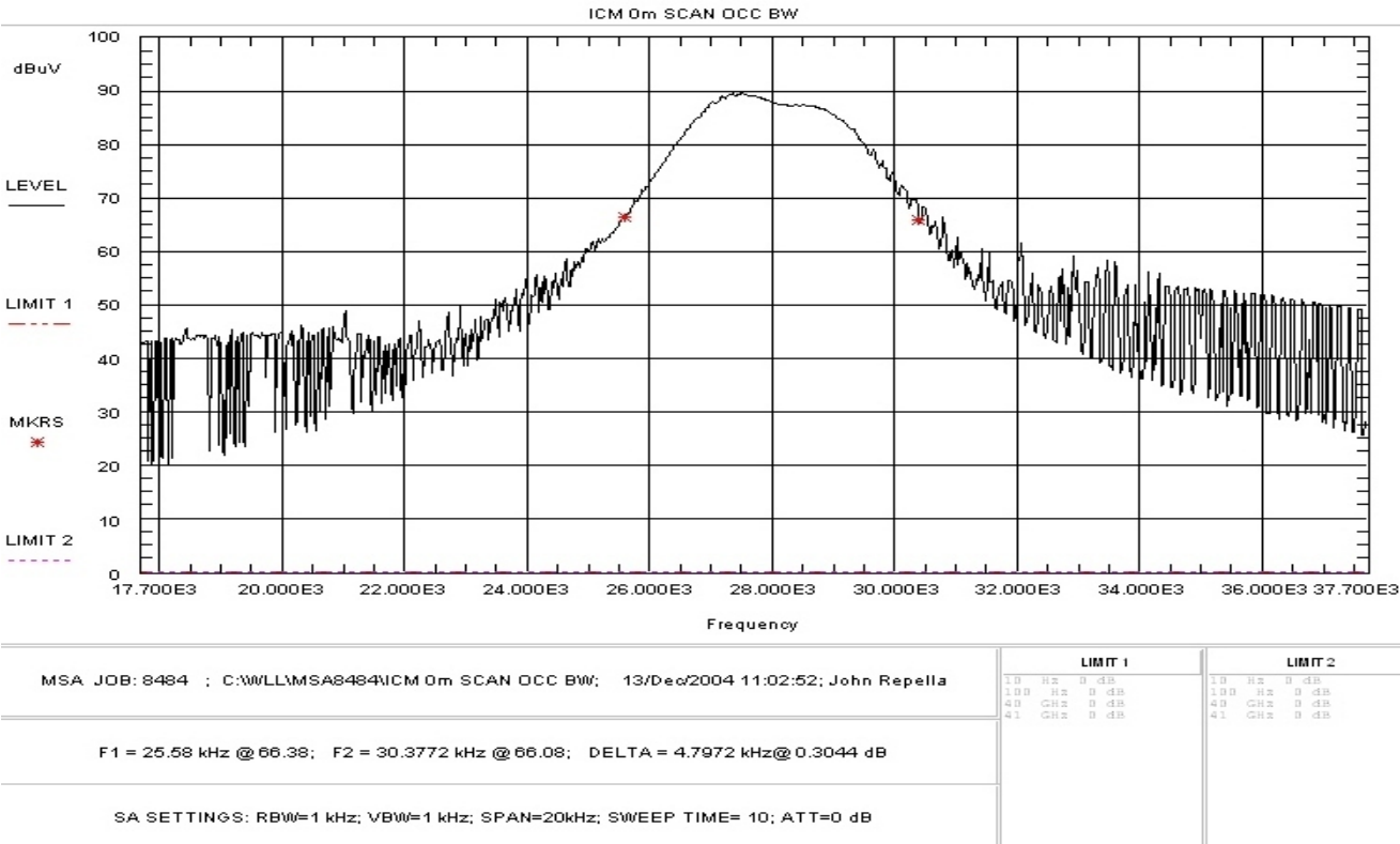
Figure 1. Occupied Bandwidth
