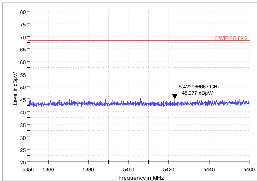
Radiated Emission Band Edge Channel No.:100 Test Mode: 802.11ac (VHT20) Polarization: H
