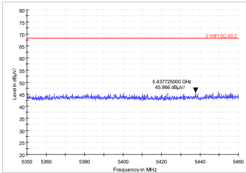
Radiated Emission Band Edge Channel No.:100 Test Mode: 802.11ac (VHT20) Polarization: V
